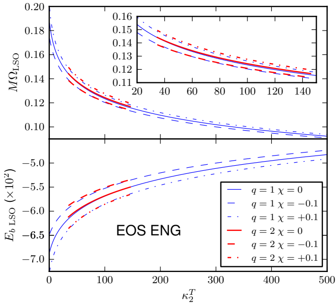
FIG. 2: GW frequency (top) and binding energy (bottom) versus the coupling constant \kappa_2^T at EOB LSO: varying mass ratio and spin magnitude. Only the ENG EOS is plotted for simplicity. The effect of mass ratio is almost negligible. The effect of spin is dominated by spin-orbit coupling.
