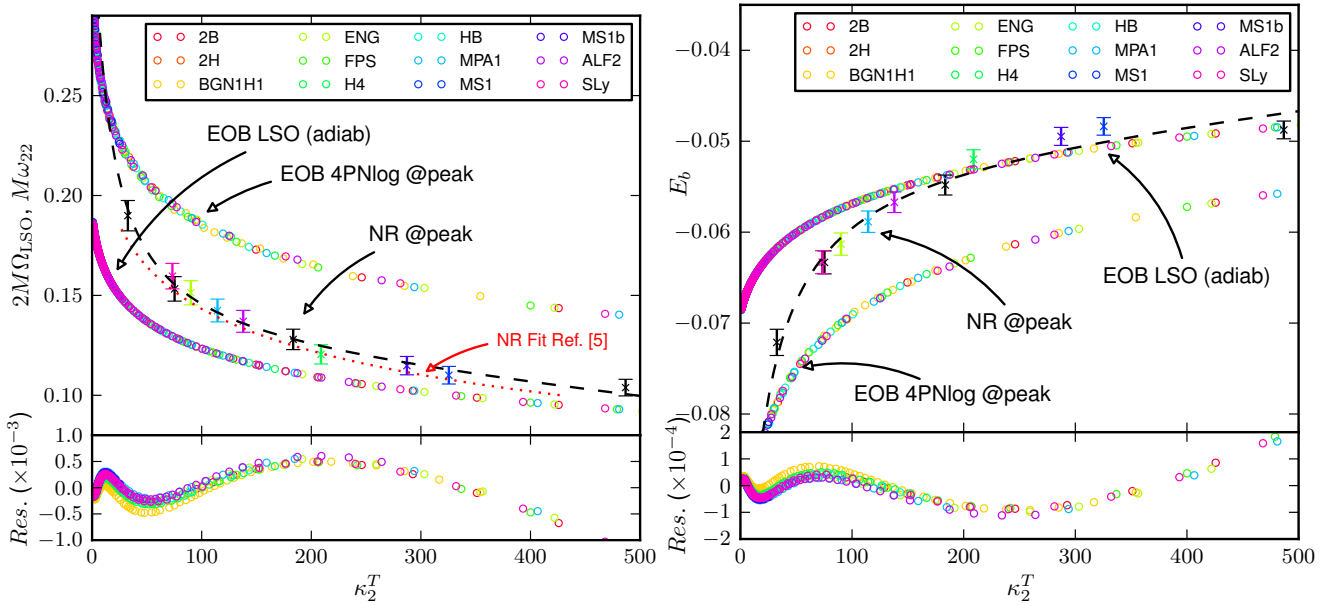
FIG. 1: GW frequency (left) and binding energy (right) versus the coupling constant \kappa_2^T for equal-masses, irrotational mergers. Main panels: Circles refer to EOB quantities computed at either the adiabatic LSO ( 2M\Omega_{\text{LSO}} , E_{b\text{LSO}} ) or the moment of merger ( M\omega_{22\text{mrg}}^{\text{EOB}} , E_{b\text{mrg}}^{\text{EOB}} ). Different colors refer to different EOS. crosses (with error bars) refer to NR quantities at the moment of merger, ( M\omega_{22\text{mrg}}^{\text{NR}} , E_{b\text{mrg}}^{\text{NR}} ). Among these, the black crosses refer to polytropic EOS. The dashed black lines are the fits given in the text. The dotted red line in the left panel is the phenomenological fit of [5]. Bottom panels: Differences in 2M\Omega_{\text{LSO}} and E_{b\text{LSO}} with respect the fits of the LSO data. An analogue result holds for the nonadiabatic EOB quantities at the moment of merger. The EOS dependence is negligible: all quantities (EOB LSO, 4PNlog EOB, and NR) show \kappa_\ell^T -universality.
