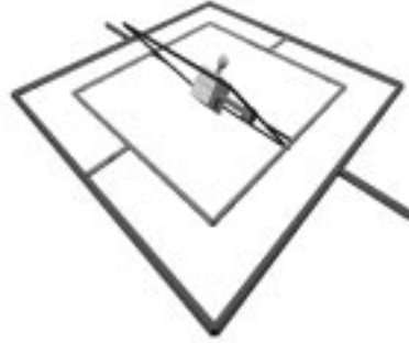
Figure 4.3: In the coordinate system the x -axis points up, the y -axis points to the left and the z -axis points to the right. In this situation the x and the z -rotation act about the same axis. This phenomenon is called gimbal lock .
