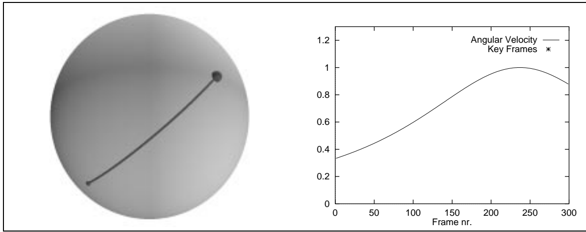
Figure 6.2: Interpolation curve and velocity graph for linear matrix interpolation — LinMat. Between the two key frames are 300 interpolated frames.
