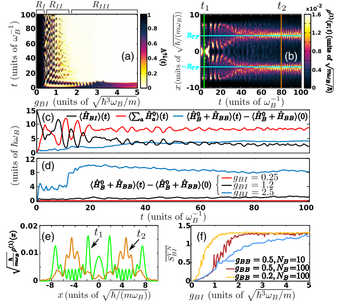
FIG. 3. (a) Evolution of the overlap \Lambda^{\uparrow\downarrow}(t) between the spin- \uparrow and spin- \downarrow states of the impurity atom. (b) One-body density evolution of the spin- \uparrow atom. Horizontal solid lines indicate the position of the Thomas Fermi radius of the bath. (c) Expectation value of the energy (see legend). In both (b),(c) g_{BI} = 1.7 . (d) Expectation value of the energy of the bath for different g_{BI} (see legend). (e) Density profiles at the time instants marked by the vertical solid lines in (b). (f) Time average of the von-Neumann entropy, \bar{S}_{BI}^{VN} , for increasing g_{BI} . In all cases N_B = 100 , N_I = 1 , and g_{BB} = 0.5 .
