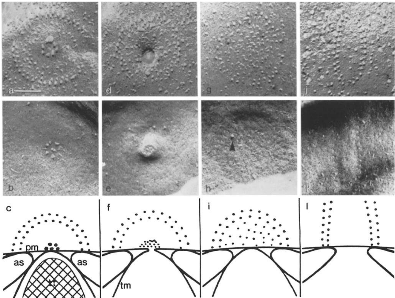
Figure 4. Ultrastructural changes in the plasma membrane during exo-endocytosis. Freeze-fracture aspects of both membrane leaflets, PF-face (top) and EF-face (middle) are depicted as representative of the categories of exo-endocytosis stages considered in the quantitative evaluation of Fig. 5. Drawings illustrate our interpretation by a combination of freeze fracture and ultrathin section aspects of docking sites (see text). as , alveolar sacs; pm , plasma membrane; tm , trichocyst membrane; tr , trichocyst tip. (a-c) Preformed exocytosis sites containing a central aggregate of rosette particles, encircled by a double ring of IMPs (on PF-faces) or pits (on EF-faces), are indicative of "resting stages" with an exocytosis-competent trichocyst docked underneath. Note also the more peripheral small b-type IMPs (Plattner et al., 1973, see also Fig. 7) within the double ring on the PF-face. Cells were mixed with water instead of AED. (d-f) Exocytotic openings are seen during the period when plasma membrane and trichocyst membrane are actually fused. Some prominent rosette particles are diffusely distributed around the exocytotic opening just formed, and several small IMPs are visible in the PF-face near the exocytotic opening. Cells were frozen 80 ms after stimulation with AED. (g-i) The resealed plasma membrane displays a round double ring filled with numerous small and "ill-defined" IMPs on the PF-face, whereas the EF-face is totally smooth. No or only a few rosette IMPs (arrowhead) are seen on either fracture face at the exocytosis sites. Cells were frozen 1,200 ms after stimulation with AED. (j-l) "Parentheses" are indicative for non-occupied exocytosis sites (after detachment of ghosts). Cells were frozen 40 s after stimulation with AED. Bar, 100 nm.
