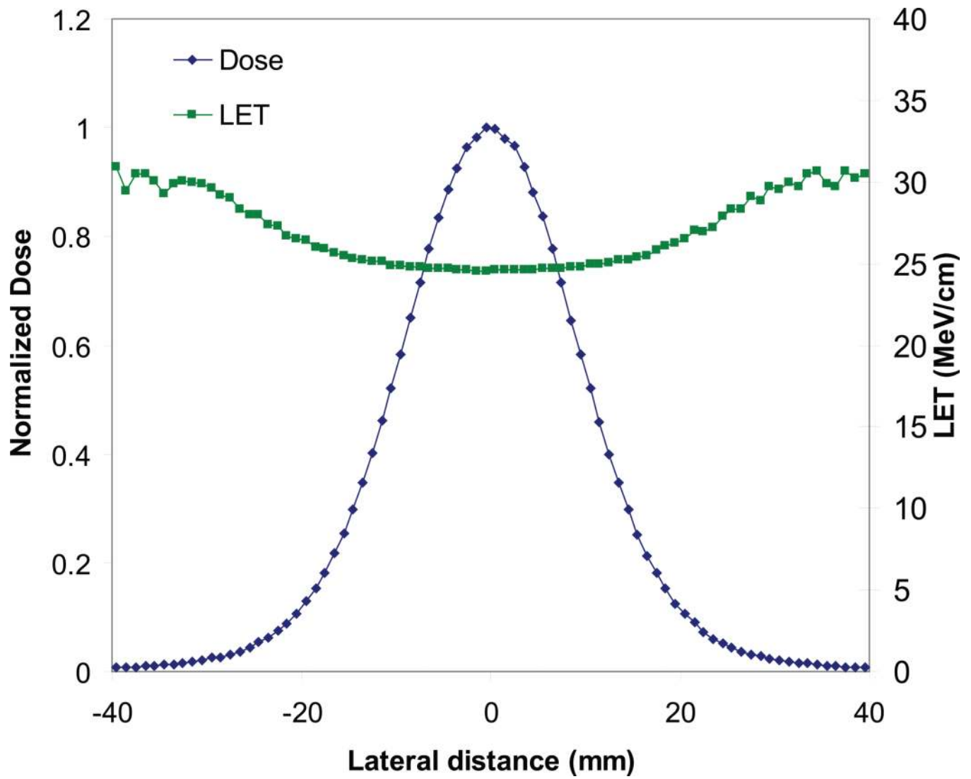
Figure 5. The Monte Carlo LET calculation shows an off-axis LET increase of up to 22% in pixels containing 1% or more of the peak dose. The lateral dose profile is shown for reference.
