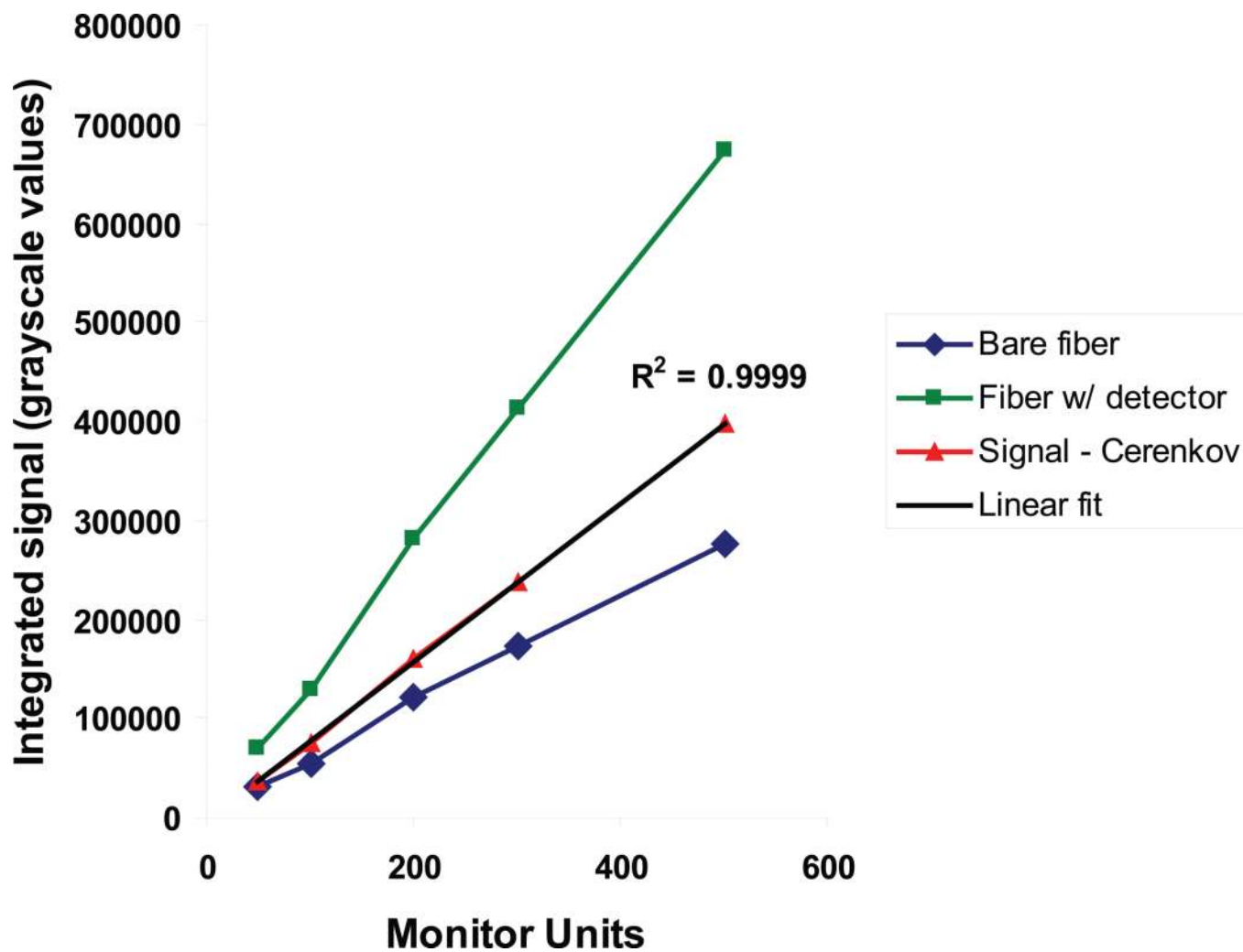
Figure 3. The results of a linearity test of a miniature LS detector in a 6-MV photon beam. The scintillation light (red) was measured by subtracting the Cerenkov signal (blue) from the miniature LS detector signal (green). The R^2 value of a linear fit to the scintillation signal was 0.9999.
