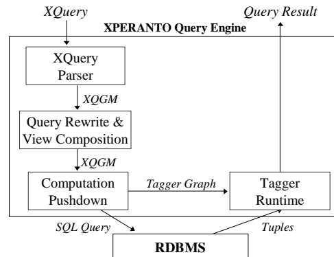
Figure 5: Query Processing Architecture
