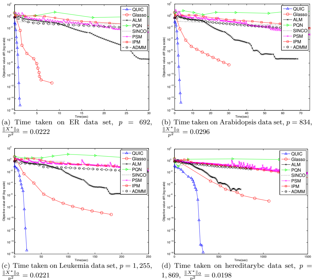
Figure 2: Comparison of algorithms on real data sets with \lambda = 0.5 . The results show that QUIC converges faster than the other methods. Notice that each marker in the figures indicates one iteration. All the results are averaged over five runs.
