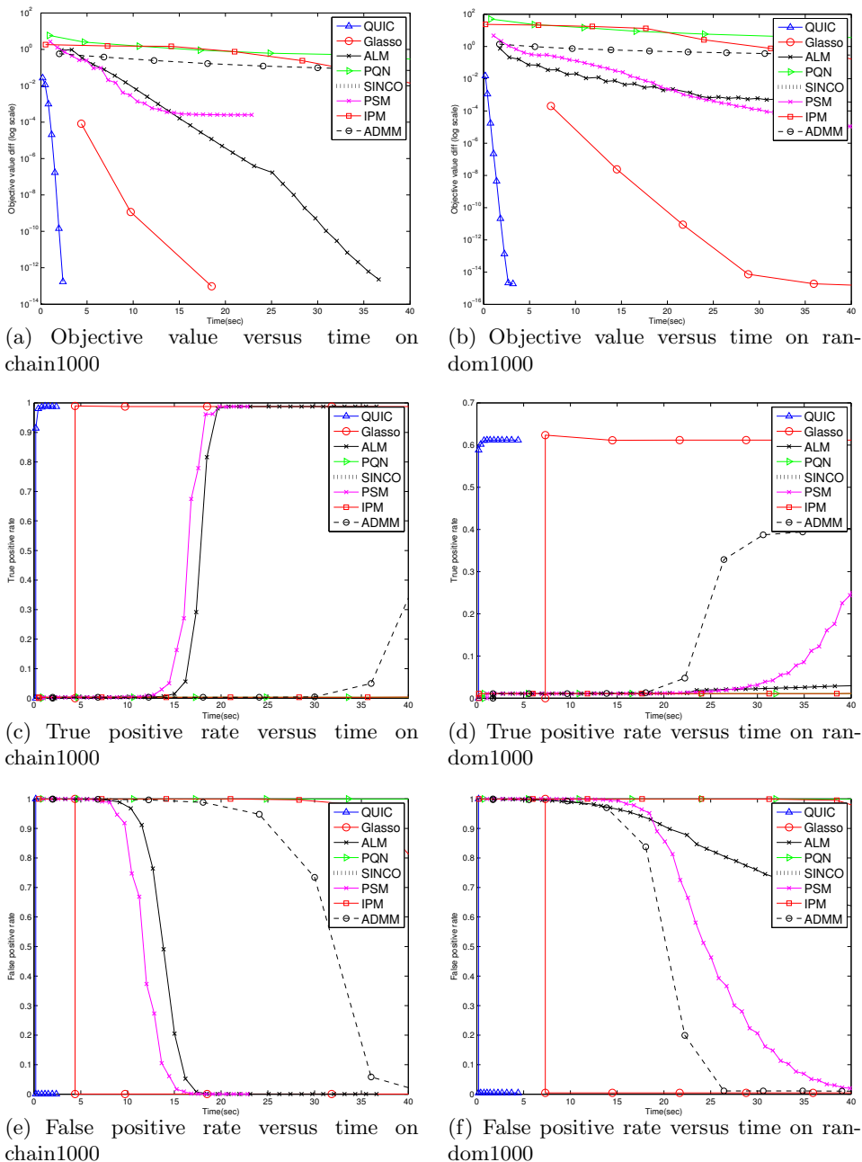
Figure 1: Comparison of algorithms on two synthetic data sets: chain1000 and random1000.
