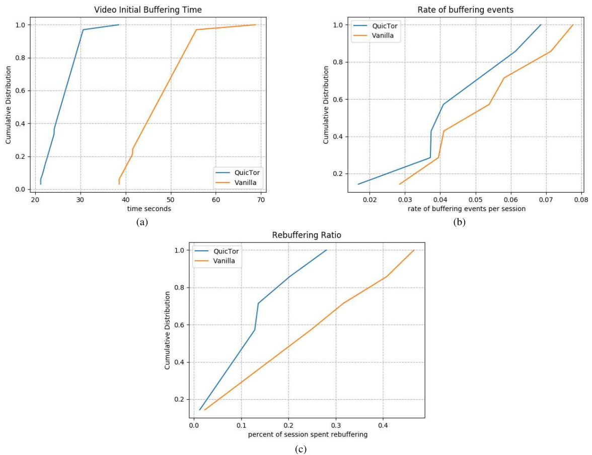
FIGURE 13. Video Streaming Performance Results.
