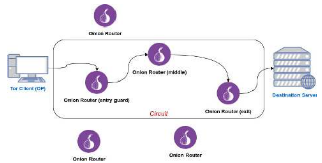
FIGURE 1. Tor network overview.
