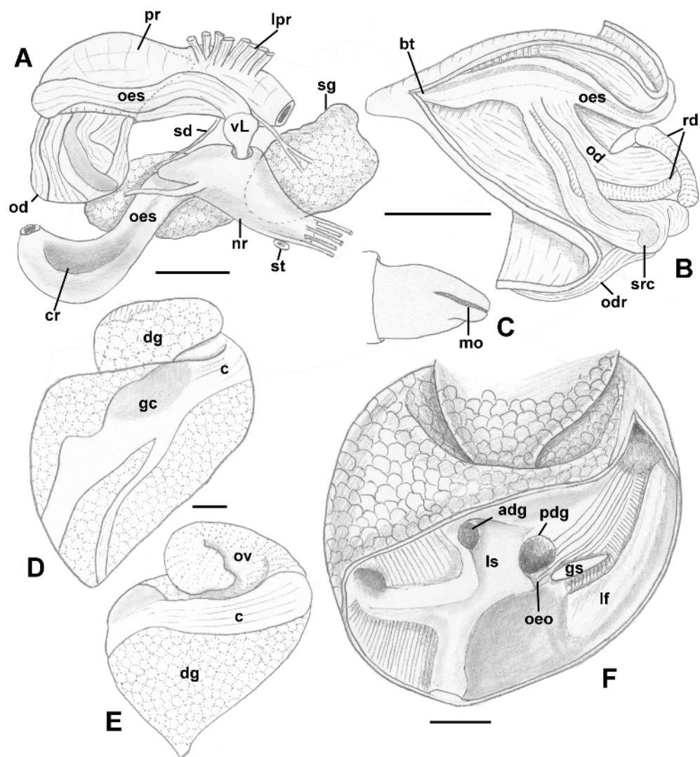
Figure 12 Anatomy of the digestive system of Nassodonta dorri . (A–C) Foregut. (A) Right view of the foregut, right salivary gland displaced to show the nerve ring, dashed line indicates proboscis retracted within rhynchodaeum. (B) Proboscis opened along left-dorsal line. (C) Proboscis tip, ventral view. (D–F) Midgut. (D–E) Views of visceral mass showing layout of posterior digestive system. (F) Gastric chamber opened along right side. adg, anterior duct of digestive gland; bt, buccal tube; c, caecum; cr, crop; dg, digestive gland; gc, gastric chamber of stomach; gs, gastric shield; lf, longitudinal fold on outer stomach wall; lpr, lateral proboscis retractors; ls, lateral sulcus; mo, mouth; nr, nerve ring; od, odontophore; odr, odontophoral retractor; oeo, esophageal opening into gastric chamber; oes, esophagus; ov, ovary; pdg, posterior duct of digestive gland; pr, proboscis; rd, radula; sd, salivary duct; sg, salivary gland; st, statocyst; vL, valve of Leiblein. Scale bars: 1 mm.
