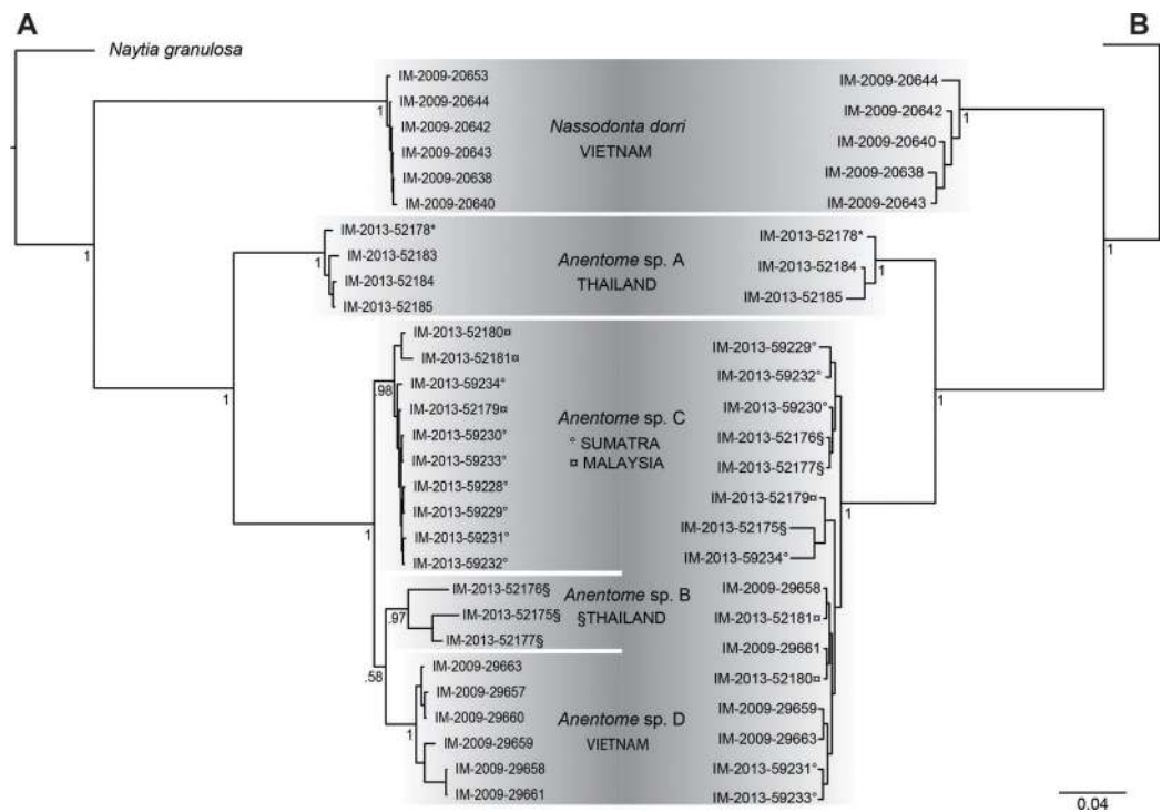
Figure 3 Bayesian phylogenies based on separate analyses of the mitochondrial and nuclear gene datasets. (A) Phylogram based on the mitochondrial gene dataset (COI, 12S, 16S). (B) Phylogram based on the nuclear gene dataset (28S, H3). Bayesian posterior probabilities are indicated at the nodes; values \geq 0.95 were considered significant. “*” indicates sequenced aquarium-trade voucher. Generic classification follows that proposed herein. See Table 1 for sources. Scale bar indicates number of nucleotide substitutions per site.
