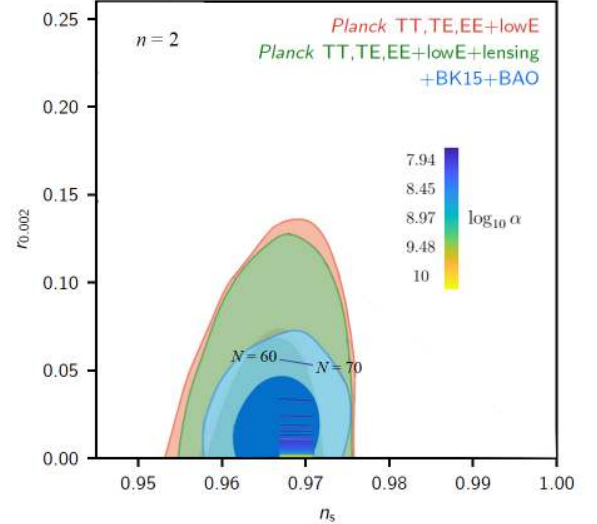
FIG. 8. r - n_s graph where the predictions derived from our model, for n = 2 , are compared to the experimental data. The number of e-folds represented range from 60 (left side) to 70 (right side). The parameter \alpha ranges from its lower bound \alpha_{\text{min}} = 8.7 \times 10^7 (blue) to \alpha = 10^{10} (yellow). Figure adapted from Ref. [39].
