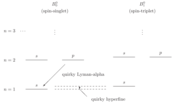
FIG. 1. Sketch of the quantum mechanical energy spectrum of our quirky dark matter composite with the ground state and several excited states shown. Our notation B_S^q corresponds to baryonic states with total electric charge q and total spin S . We have included \mathcal{O}(\bar{\alpha}^2) (quirky Lyman-alpha) and \mathcal{O}(\bar{\alpha}^4) (quirky hyperfine) splittings, but do not show the \mathcal{O}(\bar{\alpha}^5) (quirky Lamb shift) splittings or other higher-order effects. The lightest electrically charged baryons B_1^\pm (not shown), have spin one, and are slightly heavier than B_1^0 due to subdominant electromagnetic corrections to the potential.
