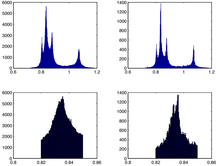
Figure 3: Value distribution of \mathfrak{R}(Q_{R,\epsilon}) and detail of the distribution for \epsilon = 10^{-2} (left) and for \epsilon = 10^{-3} (right).
