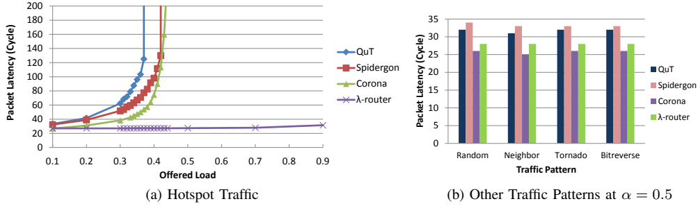
Figure 6: Average Packet Latency for 128 nodes
