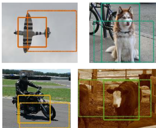
Figure 1: Some examples of the bounding box regressor outputs. The dashed box is the image-agnostic proposal, correctly selected despite the bad overlap, and the solid box is the result of improving it by using the pose regressor. Both steps use the same CNN, but the first uses the geometrically-invariant fully-connected layers, and the last the geometry-sensitive convolutional layers. In this manner, accurate object location can be recovered without using complementary mechanisms such as selective search.
