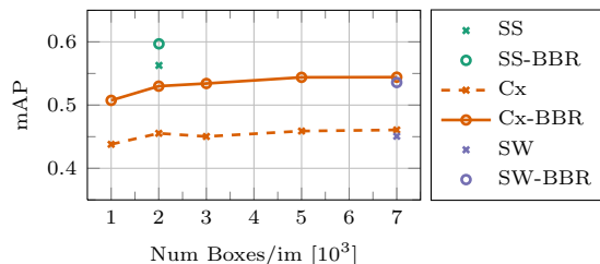
Figure 3: mAP on the PASCAL VOC 2007 test data as a function of the number of candidate boxes per image, proposal generation method, and using or not bounding box regression.
