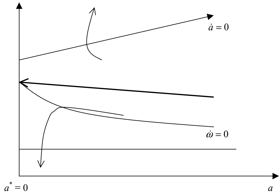
Figure 2b Steady state with growth rate \epsilon \in (0, g)
