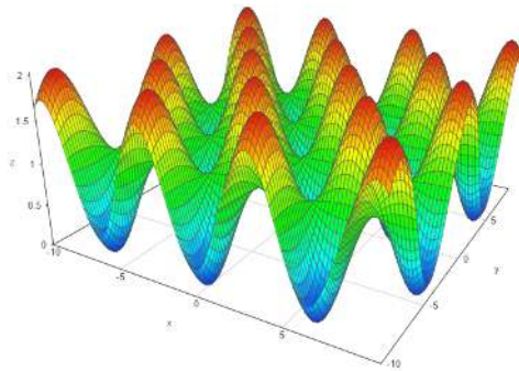
FIGURE 18. Griewank Function in a limited domain.
