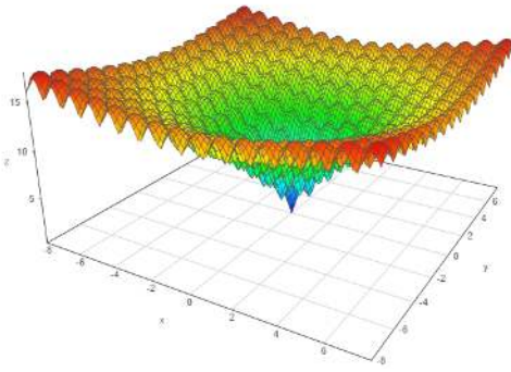
FIGURE 8. Ackley's function.
