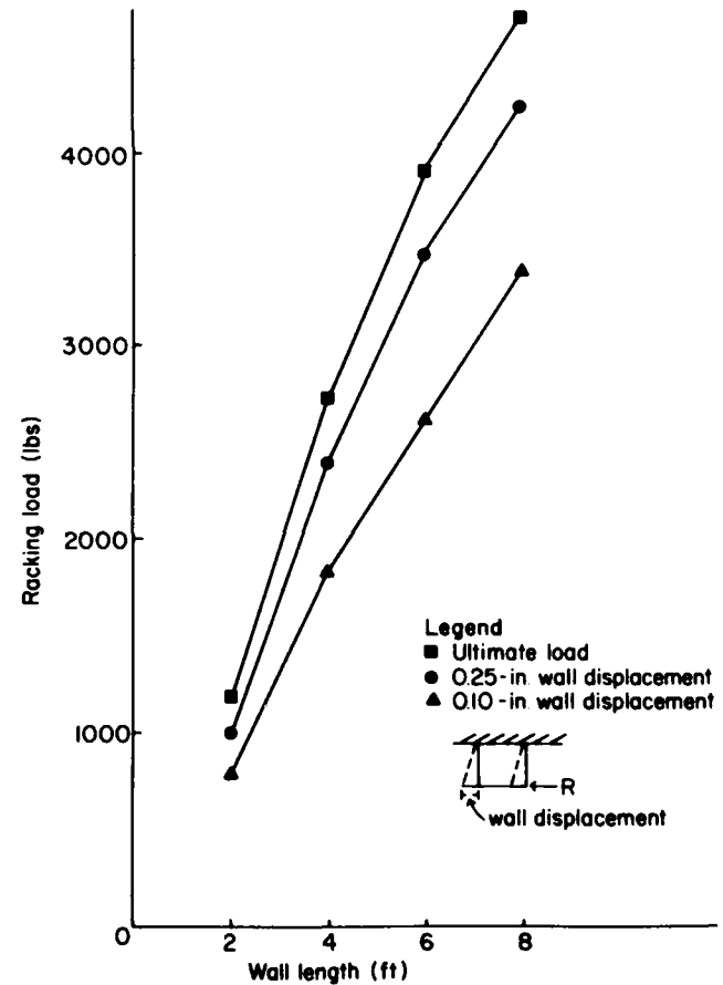
Figure 9.--Racking load versus wall length for double-sided gypsum-sheathed walls at 0.10-, 0.25-inch horizontal wall displacements and at ultimate load. (ML84 5252)
