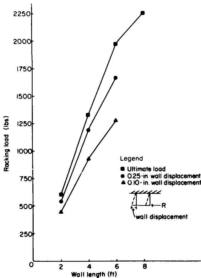
Figure 8.--Racking load versus wall length for single-sided gypsum-sheathed walls at 0.10-, 0.25-inch horizontal wall displacements and at ultimate load. (ML84 5251)
