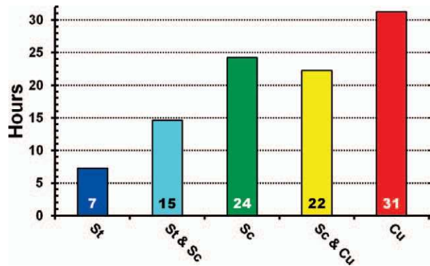
FIG. 4. RACORO flight hour distributions per cloud type. Total flight hours are plotted per cloud type sampled (or of their combinations): stratus (denoted as St), stratocumulus (denoted as Sc), and cumulus (denoted as Cu). At the base of each column, the time is expressed as a percentage of the 103 h of total cloud sampling (the percentages sum to 99% due to rounding). The cloud-type classifications are general, based on visual inspection of flight images and pilot reports.
