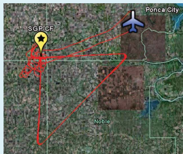
FIG. SBI. Example of a cloud flight pattern flown out of the Ponca City airport. The horizontal legs are 32 km long, and two spiral ascents were flown over the SGP.
