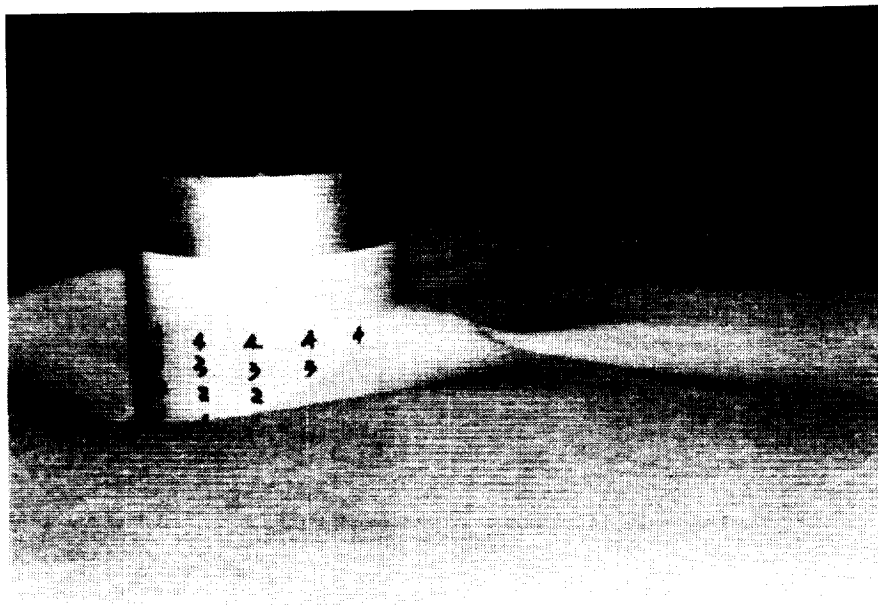
Figure 4.1c. Circular Cylinder, ISU Wind Tunnel, Height H = 10 cm, Diameter D = 10 cm, D/H = 1 , u_* = 0.73 m/s, U_h = 7.9 m/s, U_h D/\nu = 52600 , u_*^3/g\nu = 2570 , U_h t/D = 33100 , U_h^2/gD = 63.4 .
