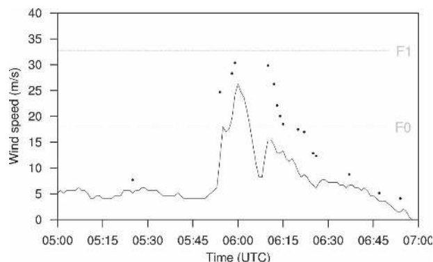
FIG. 15. As in Fig. 12, except from Harlan, IA, Automated Weather Observing Station (AWOS) during the period 0500–0700 UTC on 6 Jul 2003.
