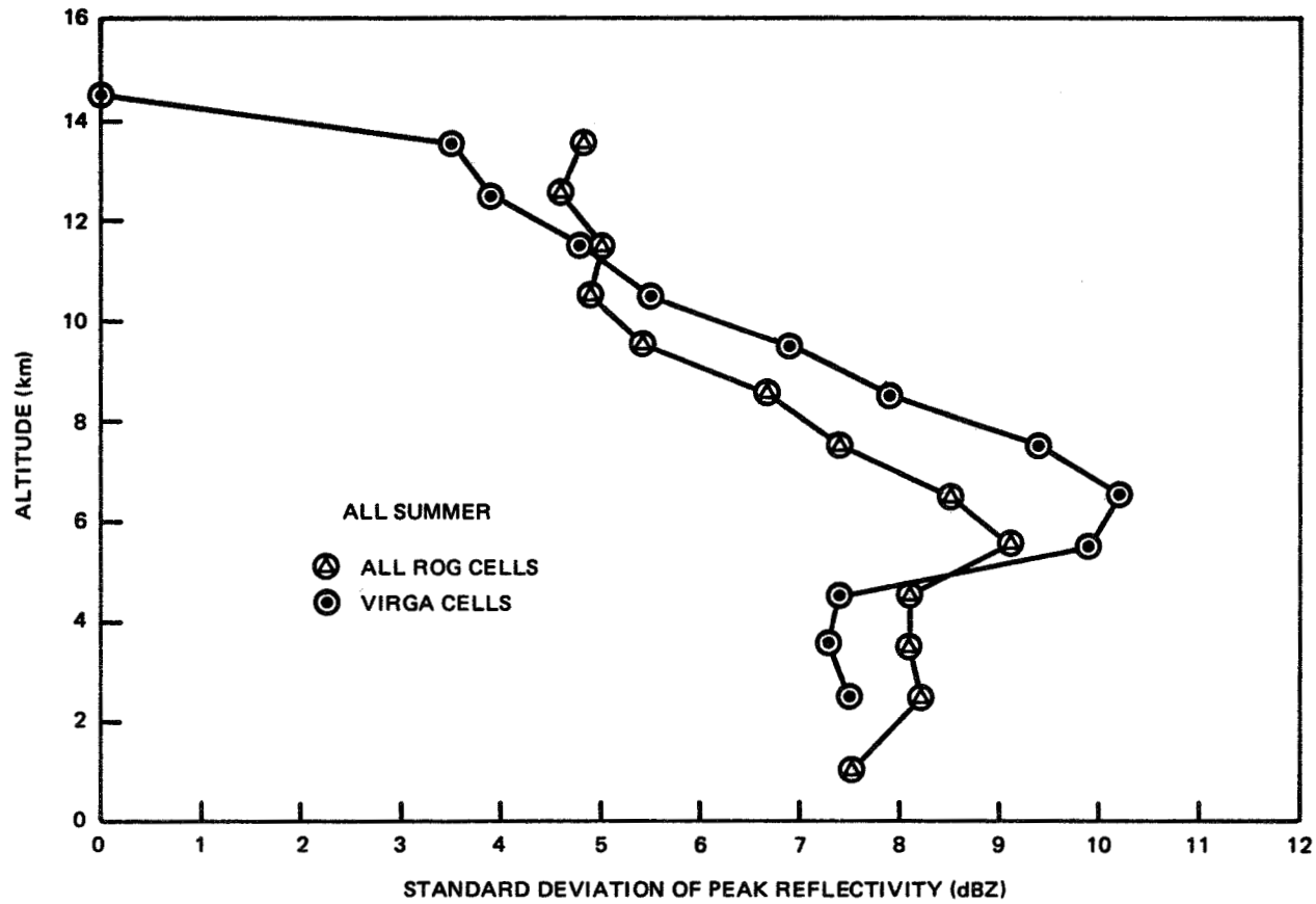
Figure 10.16. Standard Deviation of Peak Reflectivity for All ROG Class Cells and Virga
