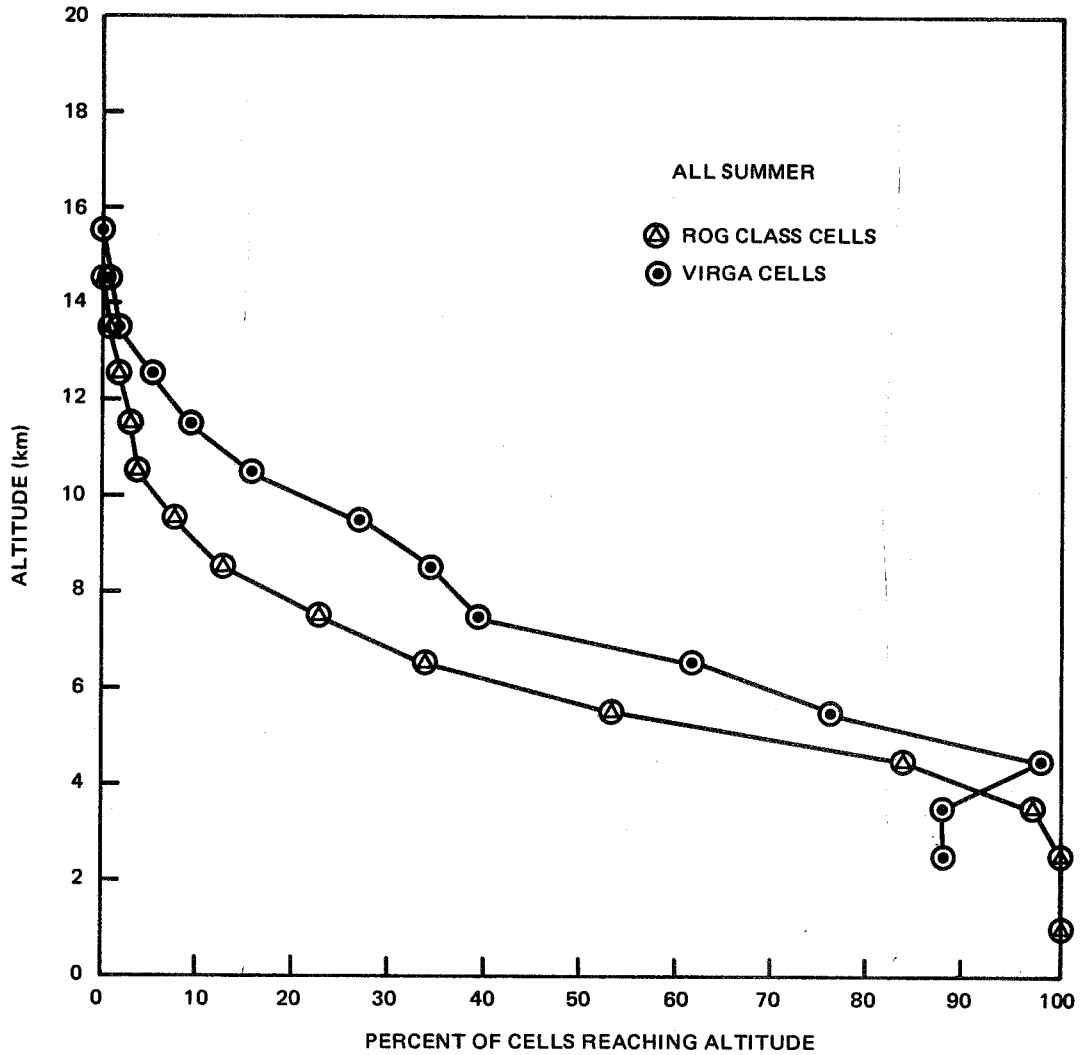
Figure 10.39. Percent of Cells Reaching Altitude for All ROG Class Cells and Virga
