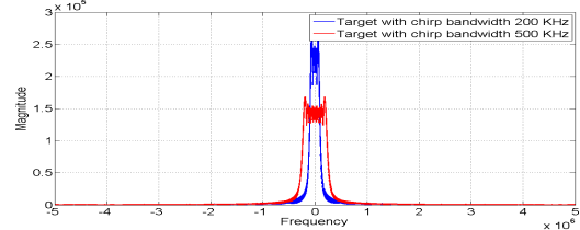
Fig. 5 FFT of different targets bandwidth
