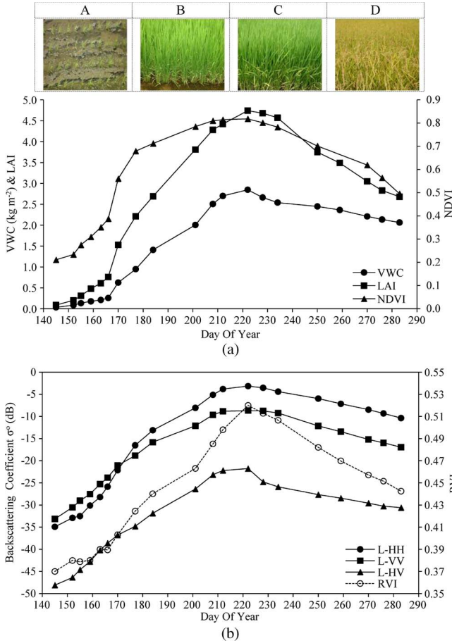
Fig. 1. Temporal variation of \sigma^{\circ} in L-band, RVI, VWC, LAI, and NDVI during the rice growth period: (a) VWC, LAI, and NDVI and (b) \sigma^{\circ} and RVI for L-band. Field photographs of rice in different growth stages: (A) Transplanting (DOY 140), (B) panicle formation (DOY 206), (C) heading (DOY 222), and (D) harvesting (DOY 283).
