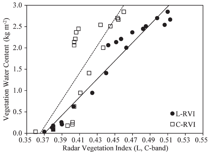
Fig. 3. Relationship between VWC and L-, C-band RVIs for rice.
