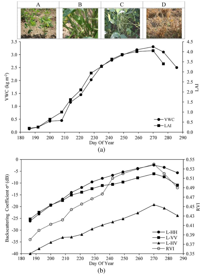
Fig. 2. Temporal variation of \sigma^{\circ} in L-band, RVI, VWC, and LAI during the soybean growth period: (a) Vegetation biophysical parameters (VWC and LAI) and (b) \sigma^{\circ} and RVI for L-band. Field photographs of soybean in different growth stages: (A) Forth trifoliolate (V4, DOY 186), (B) beginning pod (DOY 228), (C) full seed (DOY 271), and (D) harvesting (DOY 286).
