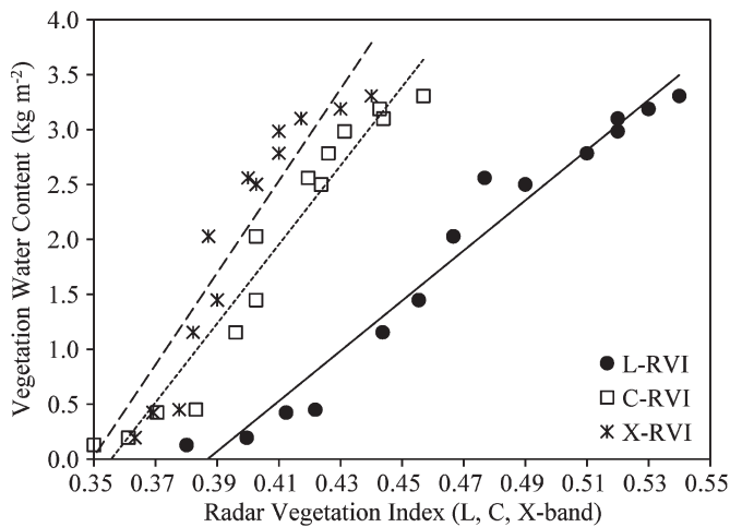
Fig. 4. Relationship between VWC and L-, C-, and X-band RVIs for soybean.
