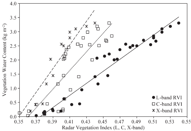
Fig. 5. Relationship between VWC and L-, C-, and X-band RVIs for rice and soybean.
