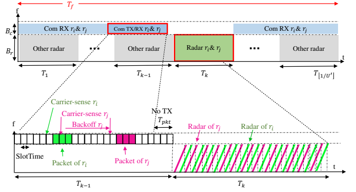
Fig. 10: RadChat Scheduling Radars scheme: FDM / rTDMA / cCSMA
