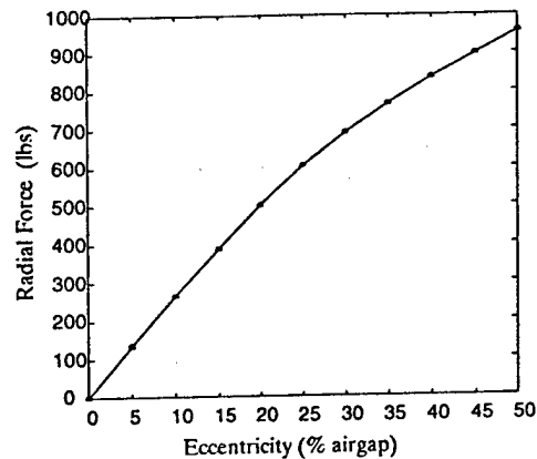
Fig. 8 Radial force -vs- eccentricity, 18/12 SRM, 90 amps and 100% alignment.
