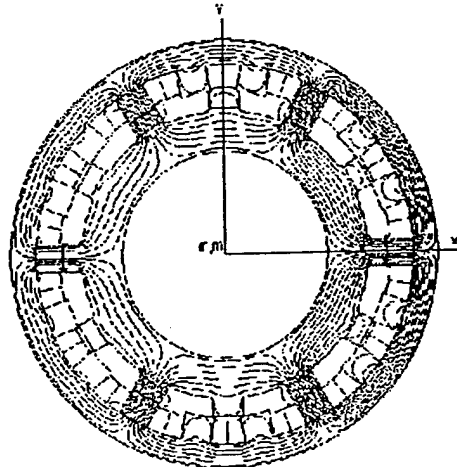
Fig. 2 FEA Flux plot for an 18/12 SRM with a 33% gap rotor offset position.
