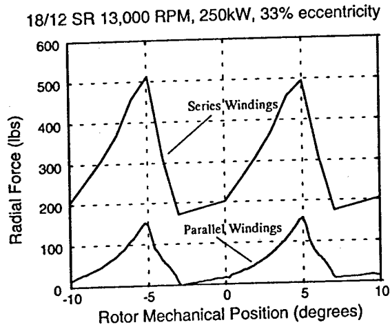
Fig. 11 Dynamic radial force comparison for voltage and current source excitation.
