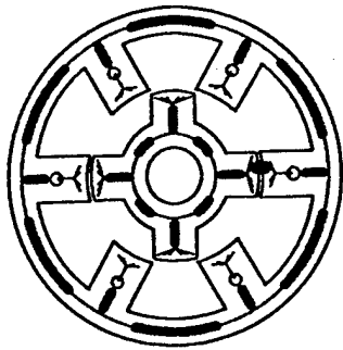
Fig. 1 Simplified MEC for 6/4 SRM
