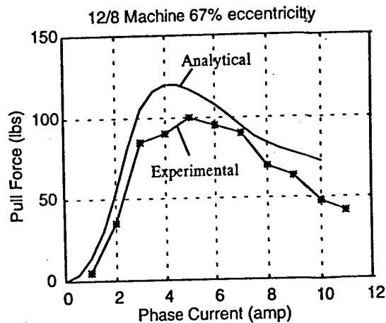
Fig. 14 Predicted and measured radial force vs. current for a 12/8 SR test machine.
