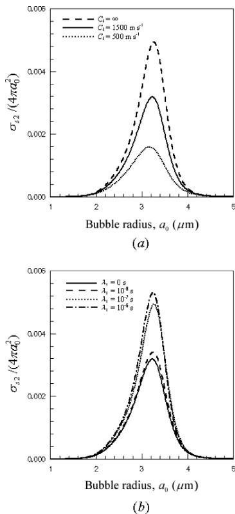
FIG. 12. Effects of (a) liquid compressibility and (b) viscoelasticity on the second-harmonic scattering cross section. The parameter P_A = 0.3 . For plot (a) \lambda_1 = \lambda_2 = 0 \text{ s} , for (b) C_l = 1500 \text{ m/s} and \lambda_2 = 0 \text{ s} .
