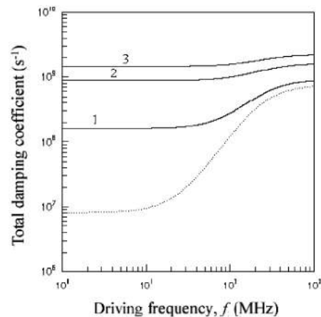
FIG. 4. Total damping coefficient as a function of driving frequency for an encapsulated microbubble of radius 1 \mu\text{m} . The curves labeled 1–3 are for values of shell thickness d = 15, 100, and 200 \text{ nm} , respectively. The total damping coefficient for a free microbubble of the same radius is marked off by the dashed line.
