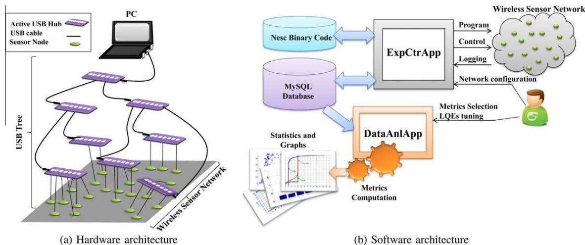
Fig. 2. RadiaLE hardware and software architectures.
