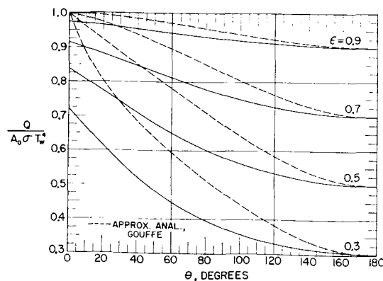
FIG. 2. Efflux of radiation through cavity opening, uniform wall temperature.
