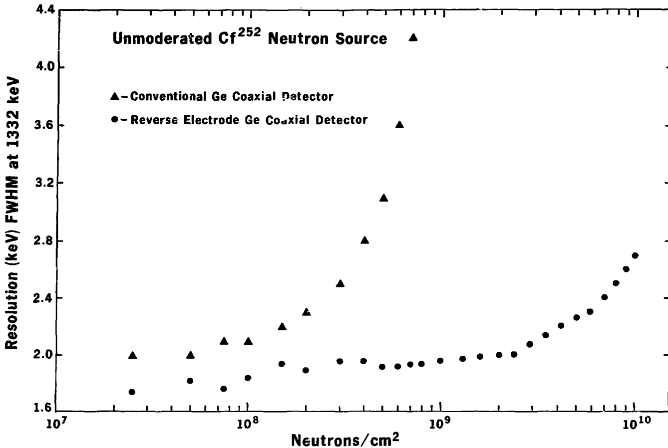
Fig. 3. Effect of neutron fluence on the energy resolution (FWHM) of the 1332 keV 60 Co line for both the conventional and reverse electrode configuration Ge coaxial detectors. Electronic noise has not been subtracted.
