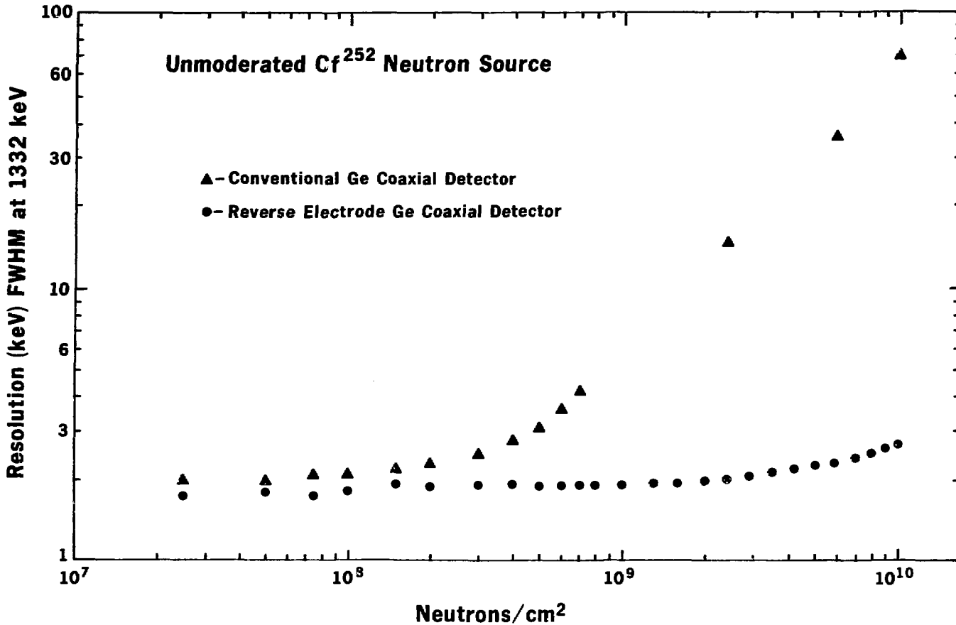
Fig. 4. Effect of neutron fluence on the energy resolution (FWHM) of the 1332 keV 60 Co line for both the conventional and reverse electrode configuration Ge coaxial detectors. Electronic noise has not been subtracted.
