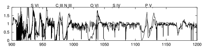
Fig. 15. Calculated and observed UV spectrum for the O4f-star \zeta Puppis. The calculated spectrum belongs to a model where the influence of shock emission has been neglected. The high resolution observations have been obtained with the IUE and Copernicus satellites. (Note that the improved blocking and blanketing treatment has not been considered for the model calculations of this object – see text.)
