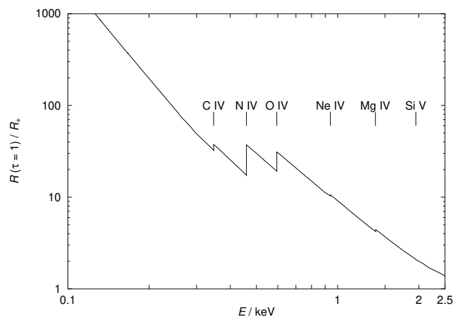
Fig. 20. Spatial location of the optical depth unity in the relevant energy band of ROSAT, displaying the origin of the observed flux. Also shown is the influence of the K-shell opacities for model 2 of \zeta Puppis.
