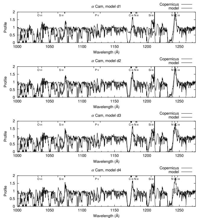
Fig. 30. Models d1–d4, a sequence in which the radius at which shocks start to form has been successively moved outwards, keeping all other parameters equal. In model d4, where Si III remains fairly unaffected by shocks, the P Cygni emission of O VI and N V has completely disappeared.
