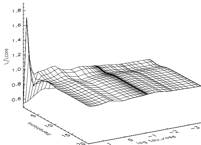
Fig. 14. The flux conservation versus the Rosseland optical depth and the iteration block number for the same O supergiant model as in Fig. 7 ( T_{\text{eff}} = 29\,000\text{ K} , \log g = 3.0 , R_*/R_\odot = 27.0 ). The accuracy of the flux conservation is on the 1% level for the final iteration blocks.
