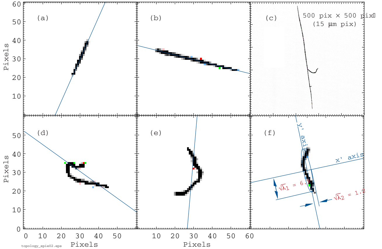
Figure 2. Examples of cosmic-ray muons (a–c) and worms (d–f) in a totally depleted 200- \mu thick LBNL CCD. (c) shows one of the longest tracks found, and two \delta rays (knock-on electrons) can be seen. (f) also indicates the the definition of \lambda_1 and \lambda_2 , the principal moments of the distribution.
