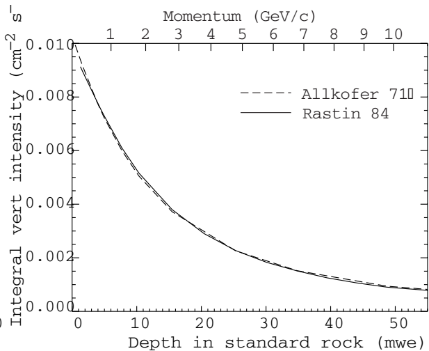
Figure 11. Integral spectrum of vertical muons as a function of depth in standard rock ( \rho = 2.65 \text{ g/cm}^3 ), expressed in meters-water-equivalent (mwe). The minimum momenta required to reach the given depths are shown by the top scale.
