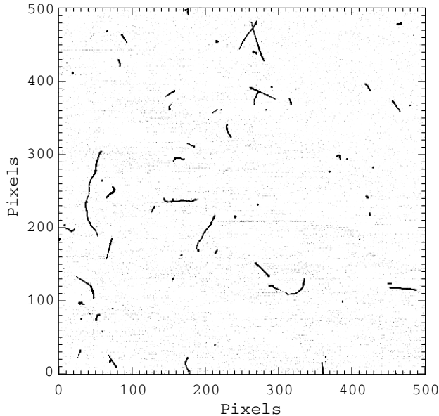
Figure 1. A 500 pixel \times 500 pixel subfield of a 4000 s dark exposure (totally depleted 200- \mu\text{m} thick LBNL CCD, Lick 3-m Coudé spectrometer room), showing cosmic-ray muons (straight tracks), worms (low-energy electrons), and spots. While the spots look insignificant, they are about as abundant as the worms and can indicate considerable deposited energy.
