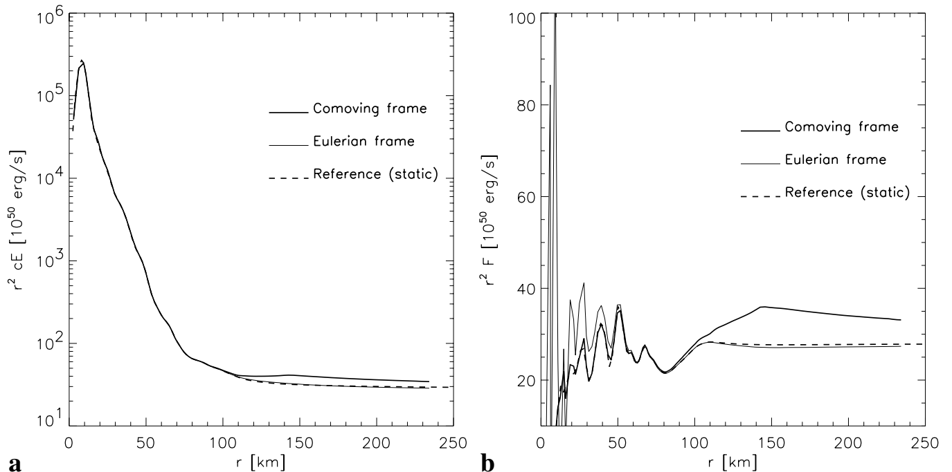
Fig. 9. Comparison of the stationary-state solutions of the comoving frame transfer equation (bold lines) with the solutions after transformation to the Eulerian frame (thin lines) and a reference calculation for a static stellar background ( v \equiv 0 ; dashed lines). Panel a ) shows the total energy density of neutrinos (times r^2 c ), Panel b ) displays the total energy flux density (times r^2 ).
