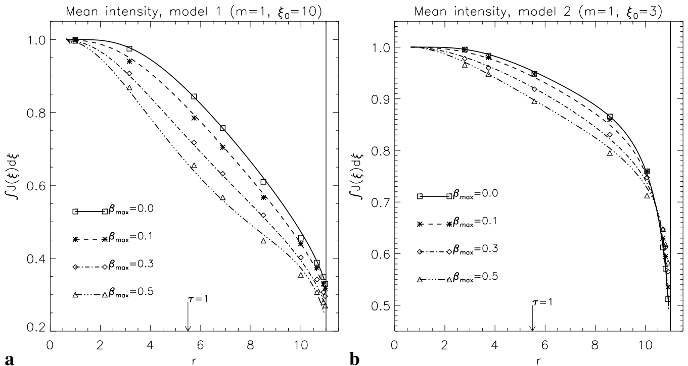
Fig. 7. Frequency integrated zeroth order angular momentum of the comoving frame intensity ( \int_0^\infty d\xi J(\xi) ) as a function of radius for our O(v/c) stationary-state solutions. The thin vertical line marks the outer boundary of the atmospheres. The small arrows point to the positions where an optical depth (which is calculated for \xi < \xi_0 ) of unity is reached. Reference solutions (symbols) obtained with a fully relativistic code were taken from Mihalas (1980, Figs. 3 and 5), where the read-off error is approximately given by the size of the symbols. Different maximum velocities \beta_{\max} of the atmospheres are indicated by different line styles and symbols. In Panel a ) the results are depicted for Model (1) with the opacity step located at \xi_0 = 10 ( \Delta = 0.25 ). Panel b ) shows results for Model (2) with \xi_0 = 3 ( \Delta = 0.2 ).
