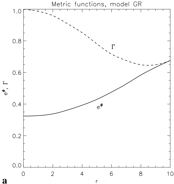
Fig. 5. Metric functions \Gamma (dashed line) and e^\Phi (solid line) of the background model (Panel a ) and stationary-state solutions for selected radiation quantities ((Panels b ), c ) versus radius. Panel b ) shows the zeroth moment J (solid line) and first moment H (dashed line) of the intensity normalized to the non-relativistic solutions. The reference solutions of Schinder & Bludman (1989) are given by the symbols ( J : triangles; H : diamonds). Error bars indicate the estimated uncertainties of reading off the reference solutions from the plots in Schinder & Bludman (1989). The Eddington factor vs. radius is shown as a solid line in Panel c ) together with the solution of Schinder & Bludman (1989, Fig. 13; diamonds).
