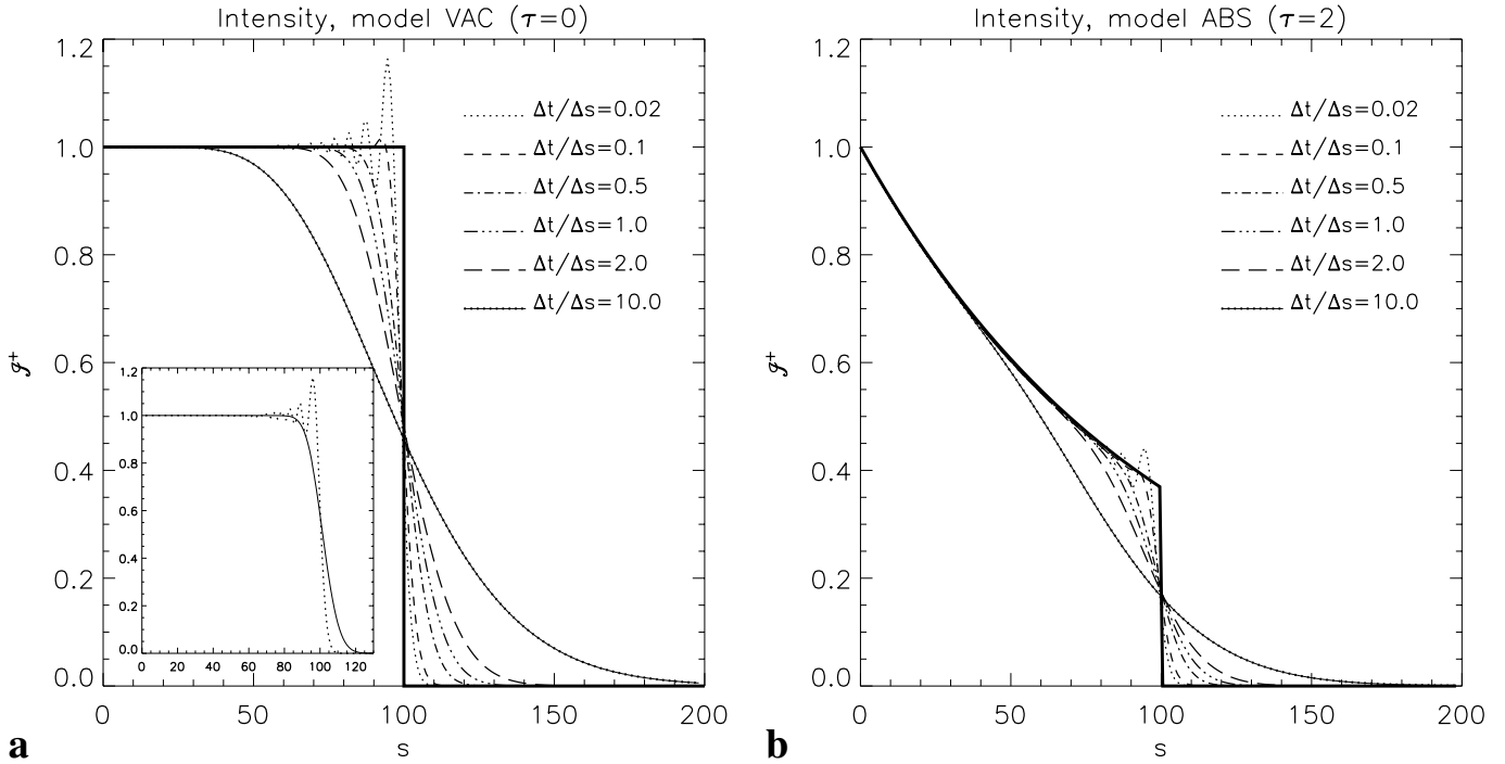
Fig. 2. Outwardly directed intensity I^+ (normalized to the true postfront value I_0 ) as a function of the position s , calculated with our Boltzmann solver at time t = 100 for different values of the computational time step. The bold line represents the analytical solution. Panel a ) shows Model “VAC” with no absorption, in Panel b ) Model “ABS” with the absorptive shell is displayed. Employing an additional diffusive term in the transport equations helps damping the spurious post-front oscillations, which are most prominent for \Delta t/\Delta s = 0.02 (cf. the solid line compared to the dotted line in the plot inserted in Panel a )).
