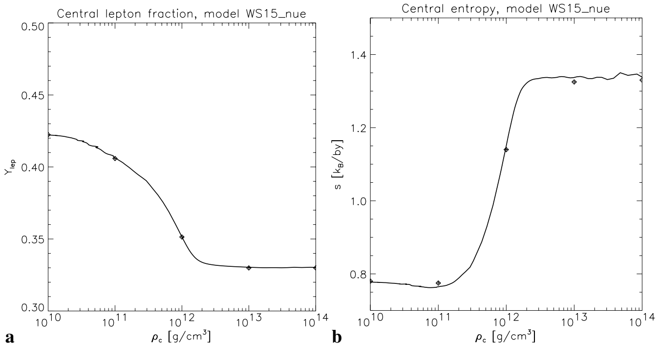
Fig. 11. Central lepton fraction Y_{\text{lep}} := Y_e + Y_{\nu_e} (Panel a ) and central entropy per baryon ( b ) as functions of the central density for our Newtonian core-collapse simulation of a 15 M_{\odot} star (solid lines), compared with the results (diamonds) obtained by Bruenn & Mezzacappa (1997, Figs. 4a, 8a).
