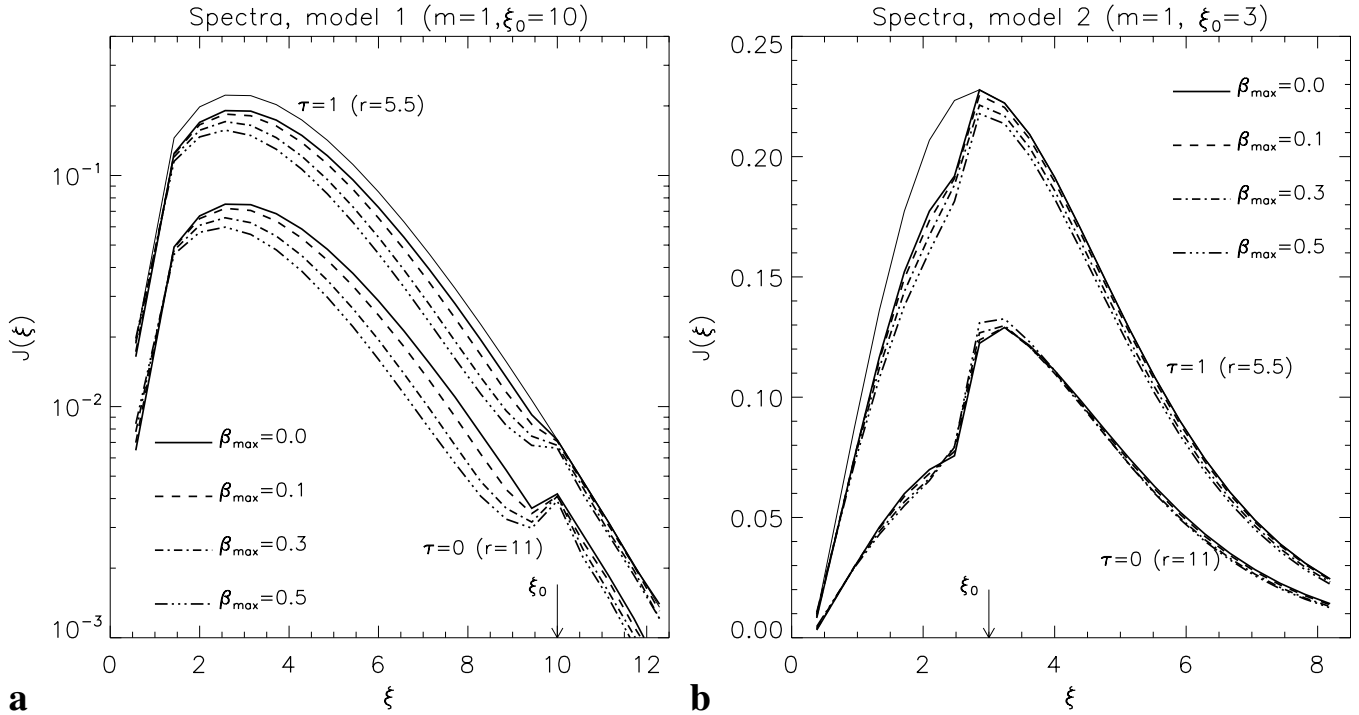
Fig. 8. Spectral distributions of the angular momentum J of the comoving frame intensity for our stationary-state solutions of the O(v/c) radiative transfer equation. Spectra are displayed for a radial position corresponding to an optical depth (which is calculated for \xi < \xi_0 ) of unity and for the surface of the atmosphere. For comparison, the equilibrium intensity (Planck function) at an optical depth of unity is plotted as a thin line. Different maximum velocities ( \beta_{\max} ) of the expanding atmospheres are indicated by different line styles. Panel a ) shows results for Model (1), where the opacity step (vertical arrows in the plots) is located at \xi_0 = 10 ( \Delta = 0.25 ). Panel b ) shows Model (2) with \xi_0 = 3 ( \Delta = 0.2 ). Our results may be compared with Mihalas (1980, Figs. 4 and 6).
