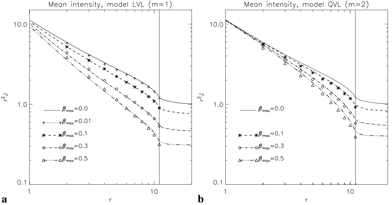
Fig. 6. Stationary-state angular mean J (times r^2 ) of the intensity as measured in the comoving frame of reference. The abscissa gives the radial position. Results are shown for gray scattering atmospheres that expand according to a linear (Model “LVL”; Panel a ) and the quadratic (Model “QVL”; Panel b ) velocity law. The thin vertical line marks the upper boundary of the atmospheres. Different line styles of the curves correspond to different values of the parameter \beta_{\max} which gives the maximum expansion velocity in units of c reached at the surface ( r = 11 ) of the model atmospheres. The thin solid curve corresponds to the static case. Reference solutions (symbols) were taken from Mihalas (1980, Fig. 2).
