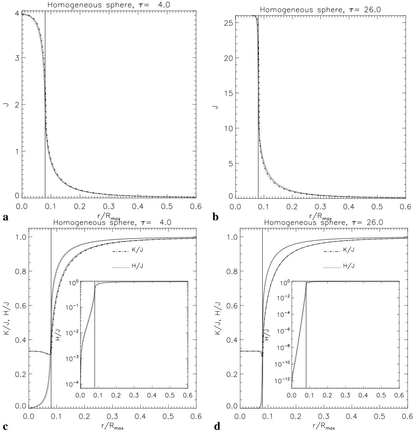
Fig. 3. Numerical (dotted and dash-dotted lines) and analytical (solid lines) stationary-state solutions vs. radius (normalized to the radius R_{\max} of the outer boundary) of homogeneous sphere problems with “low” ( \tau = 4 , left column, Panels a , c ) and “high” opacity ( \tau = 26 , right column, Panels b , d ). Panels a ) and b ) show the zeroth moment of the intensity. In Panels c ) and d ) the Eddington factor K/J (dash-dotted) and the flux factor H/J (dotted) are displayed. The inserted panels show the flux factor on a logarithmic scale. Thin vertical lines mark the surface R of the homogeneous sphere.
