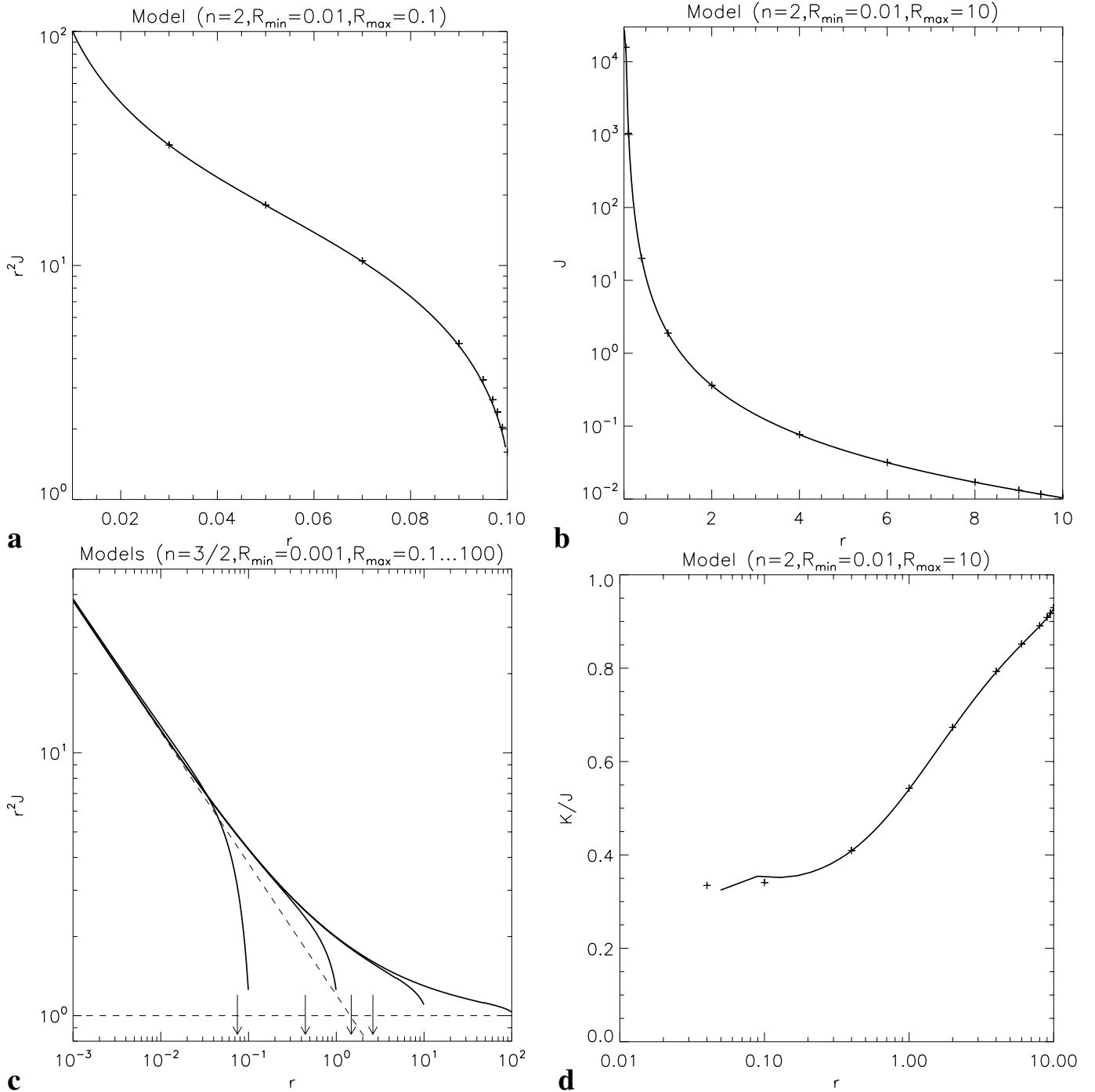
Fig. 4. Stationary state solutions for selected radiation quantities as a function of radius obtained with our radiative transfer code (solid lines). Our results are compared with the reference solutions (crosses) and asymptotic solutions (dashed lines) of Hummer & Rybicki (1971). Panel a ): mean intensity J (times r^2 ) for the combination of model parameters (n = 2, R_{\min} = 0.01, R_{\max} = 0.1) ; Panel b ): mean intensity J for (n = 2, R_{\min} = 0.01, R_{\max} = 10) ; Panel c ): r^2 J for models with (n = 3/2, R_{\min} = 0.001, R_{\max} \in \{0.1, 1, 10, 100\}) . The vertical arrows indicate the radial positions, where \tau = 1 is reached in the different atmospheres; Panel d ): Eddington factor K/J for the test case with a purely radial distribution of the radiation intensity at the inner boundary and the model parameters (n = 2, R_{\min} = 0.01, R_{\max} = 10) . Note that the solid line connects values which are evaluated at the centers of the radial zones of our computational grid, the first one being located at r_{\frac{1}{2}} = 0.05 .
