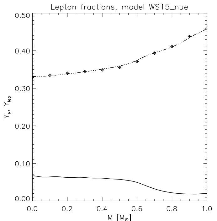
Fig. 10. Profiles of the total lepton fraction Y_{\text{lep}} (dash-dotted line) and the electron neutrino fraction Y_{\nu_e} (solid line) as a function of the enclosed mass at the time when the central density reaches 10^{14} \text{ g cm}^{-3} . For comparison the results of Bruenn & Mezzacappa (1997, Fig. 5a) are plotted with diamonds.
