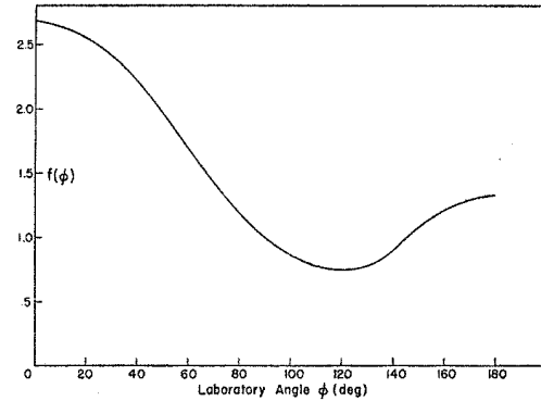
FIG. 6. Angular dependence of nonrelativistic limit of U^{(\Omega)} (without \ln \lambda term).
