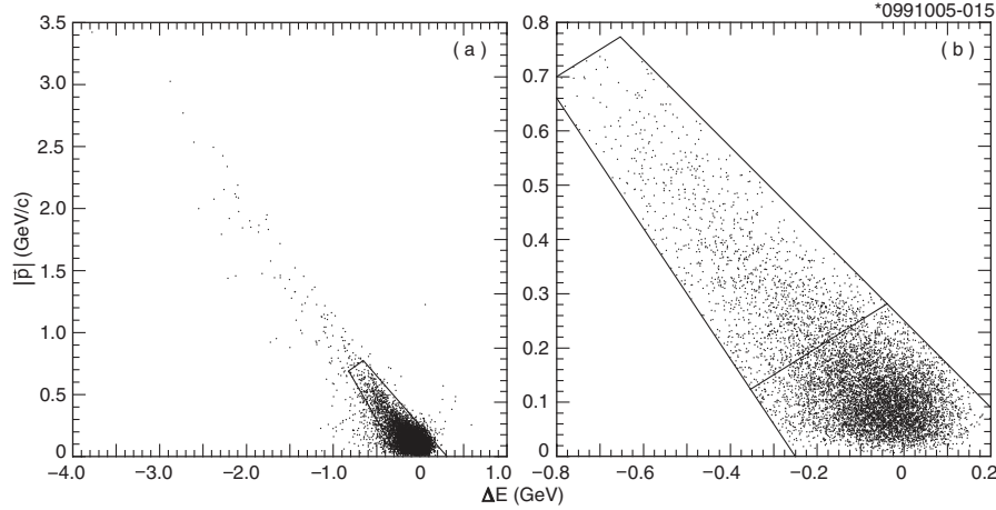
FIG. 1. Illustration of the chosen 4-momentum distribution cuts on a larger (a) and smaller (b) scale, using Monte Carlo events for the decay channel Y(1S) \rightarrow \gamma f_2(1270) \rightarrow \gamma \pi^0 \pi^0 . The slanted line in the lower right part of (b) divides the selected events roughly into two categories: the lower area where the 4-momentum is conserved for the entire event; the upper area where the 4-momentum is conserved for the intermediate resonance but not for the entire event. The remaining events outside the selected area in (a) have an energy loss from more than one photon and, hence, are excluded from the selection.
