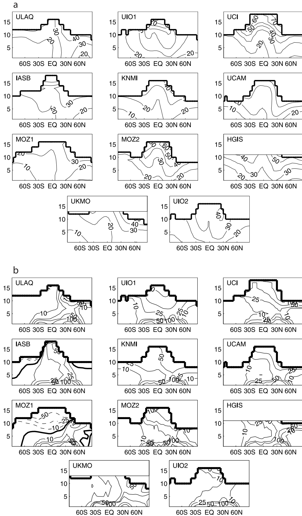
Figure 2. Increase in annually averaged zonal mean (a) ozone and (b) NO x between 2000 and 2100 (year 2100 values minus year 2000 values). All models in this figure used fixed ozone levels, ozone flux, or ozone precursor levels in the stratosphere. Contour lines at 10, 20, 30, 40, 50, 60, 70, and 80 ppbv (Figure 2a), and at -100, -50, -25, 0, 10, 25, 50, 100, 250, 500, and 1000 pptv (Figure 2b) (negative contour lines dashed). As in IPCC-TAR, grid boxes with (year 2000) ozone mixing ratios above 150 ppbv are masked. The altitude is given in kilometers.
