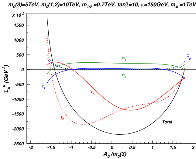
FIG. 2 (color online). Plot of third generation contributions to \Sigma_u^u versus A_0 for benchmark point RNS1 where solid curves come from the lighter mass eigenstate and dashed curves from the heavier. The black solid curve labelled “total” is \Sigma_u^u which has summed over all contributions.
