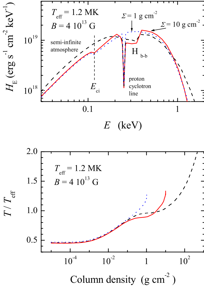
Fig. 12. Comparison of emergent spectra ( top panel ) and temperature structures ( bottom panel ) of the fiducial model (solid curves) with the semi-infinite model atmosphere (dashed curves) and with the thinner ( \Sigma = 1 g cm -2 ) model atmosphere (dotted curves), but with the same magnetic field.
