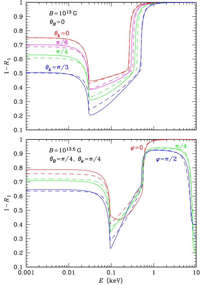
Fig. 6. Dimensionless emissivity for the linear polarization e_1 , J_1 = 1 - R_1 , as a function of photon energy E for condensed Fe surface at different magnetic field strengths and geometric settings. Top panel: magnetic field B = 10^{13} G is normal to the surface, and angles of radiation incidence are \theta_k = 0, \pi/6, \pi/4 , and \pi/3 . Bottom panel: B = 10^{13.5} G, magnetic field lines and the photon beam are both inclined at \theta_B = \theta_k = \pi/4 , and the azimuthal angle takes values \varphi = 0, \pi/4 , and \pi/2 . Solid lines show the numerical results, and dashed lines demonstrate the fit.
