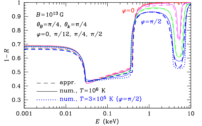
Fig. 4. Dimensionless emissivity J = 1 - R as a function of photon energy E for a condensed Fe surface with inclined magnetic field ( B = 10^{13} G, \theta_B = \pi/4 , \theta_k = \pi/4 ) and inclined incidence of radiation ( \theta_k = \pi/4 and four values of \varphi listed in the figure). Solid lines show our numerical results for the model of free ions at T = 10^6 K, and short-dashed lines demonstrate the fit. For comparison, the dotted line reproduces our numerical results for \varphi = \pi/2 and T = 3 \times 10^5 K.
