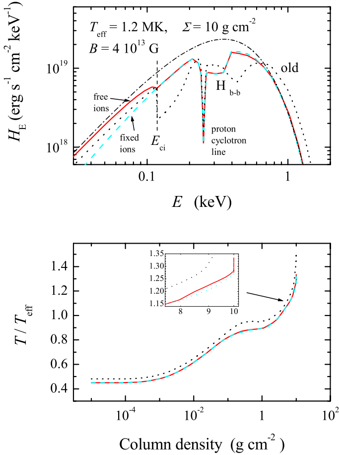
Fig. 8. Emergent spectra ( top panel ) and temperature structures ( bottom panel ) for the fiducial model atmosphere (solid curve) and for model atmospheres that are calculated using the fixed-ions approximation for the reflectivity calculations (dashed curves), and the inner boundary condition from Paper II (dotted curves). In the top panel the diluted blackbody spectrum that fits the high-energy part of the fiducial model spectrum is also shown (dash-dotted curve).
