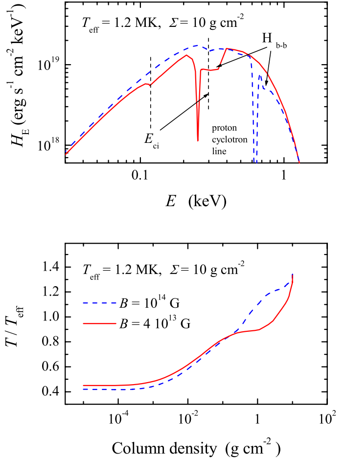
Fig. 13. Comparison of emergent spectra ( top panel ) and temperature structures ( bottom panel ) of the fiducial model (solid curves) and the model atmosphere with different magnetic field ( B = 10^{14} G), but with the same surface density (dashed curves).
