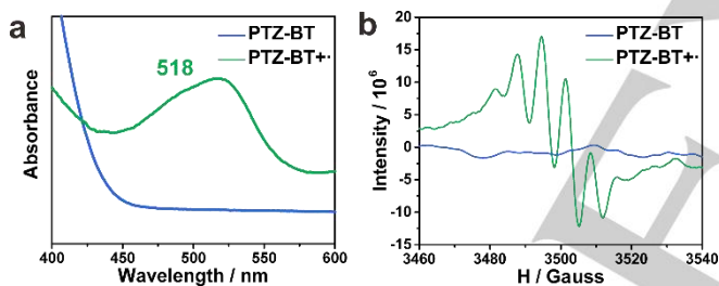
Figure 1. The (a) UV-Vis absorption spectra and (b) ESR spectra of PTZ species in THF/TMB mixed solution, before (blue) and after (green) the addition of TFA.
