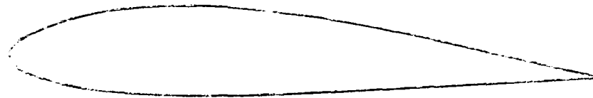
NACA 64 2 - 415 AIRFOIL
