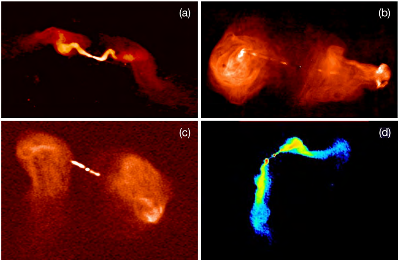
Figure 1. Four examples of various radio-loud galaxy morphologies. (a) FR-I radio source 3C31 at 1.4 GHz with the VLA from NRAO/AUI ( http://images.nrao.edu/AGN/Radio_Galaxies/ ) by R. Laing, A. Bridle, R. Perley, L. Feretti, G. Giovannini and P. Parma (Laing 1996). (b) 3C353 at 8.4 GHz with the VLA from NRAO/AUI by M. Swain, A. Bridle and S. Baum (Swain, Bridle & Baum 1998). (c) 3C288 at 8.4 GHz with the VLA from NRAO/AUI by A. Bridle, J. Callcut and E. Fomalont (Bridle et al. 1989). (d) A WAT radio source, 3C465, in Abell 2634 at 1.4 GHz with the VLA from the Atlas of DRAGNs ( http://www.jb.man.ac.uk/atlas/object/3C465.html ) by F. Owen (Eilek et al. 1984; Leahy et al. 1996).
