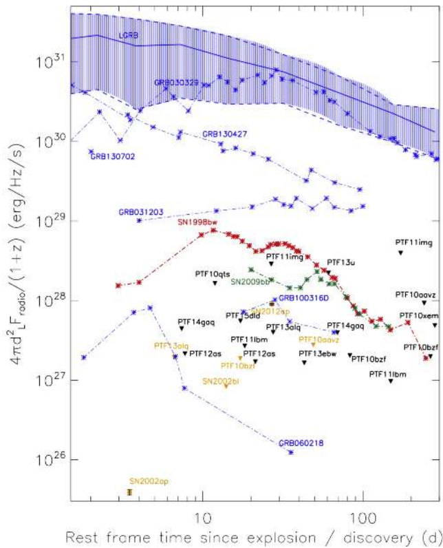
Figure 4. Radio (observed central frequencies of \approx 4.8\text{--}6.3 GHz; see Table 3) upper limits for the BL-Ic SNe in our sample with VLA follow-up observations at t \lesssim 300 days since discovery (as measured in the SN rest frame), compared with: the mean radio (8.5 GHz) light curve of cosmological GRBs (blue solid line) as derived by Chandra & Frail (2012), together with the 75% confidence interval (blue shaded region); radio ( \sim 5 GHz) afterglow light curves of long GRBs with spectroscopically associated SNe (blue asterisks; Berger et al. 2003b; Soderberg et al. 2004; Frail et al. 2005; Soderberg et al. 2006c; Margutti et al. 2013; Perley et al. 2014; Singer et al. 2015); the light curve of the GRB-SN 1998bw (red asterisks; Kulkarni et al. 1998); the light curve of the relativistic BL-Ic SN 2009bb (green asterisks; Soderberg et al. 2010), and SN 2012ap (yellow dot; Chakraborti et al. 2015; Milisavljevic et al. 2015). Black triangles are our upper limits. Yellow data points, or upper limits, are for BL-Ic SN radio ( \sim 5\text{--}8.5 GHz) follow-up observations that were not conducted via our programs (Berger et al. 2003a; Chomiuk & Soderberg 2010; Soderberg et al. 2010; Soderberg & Chomiuk 2011; Kamble & Soderberg 2013). Radio detections for the PTF sample are plotted in Figure 5. Late-time radio observations of BL-Ic SNe performed at t \gtrsim 300 days since explosion via other studies (Soderberg et al. 2006b; Bietenholz et al. 2014) are not reported here.
