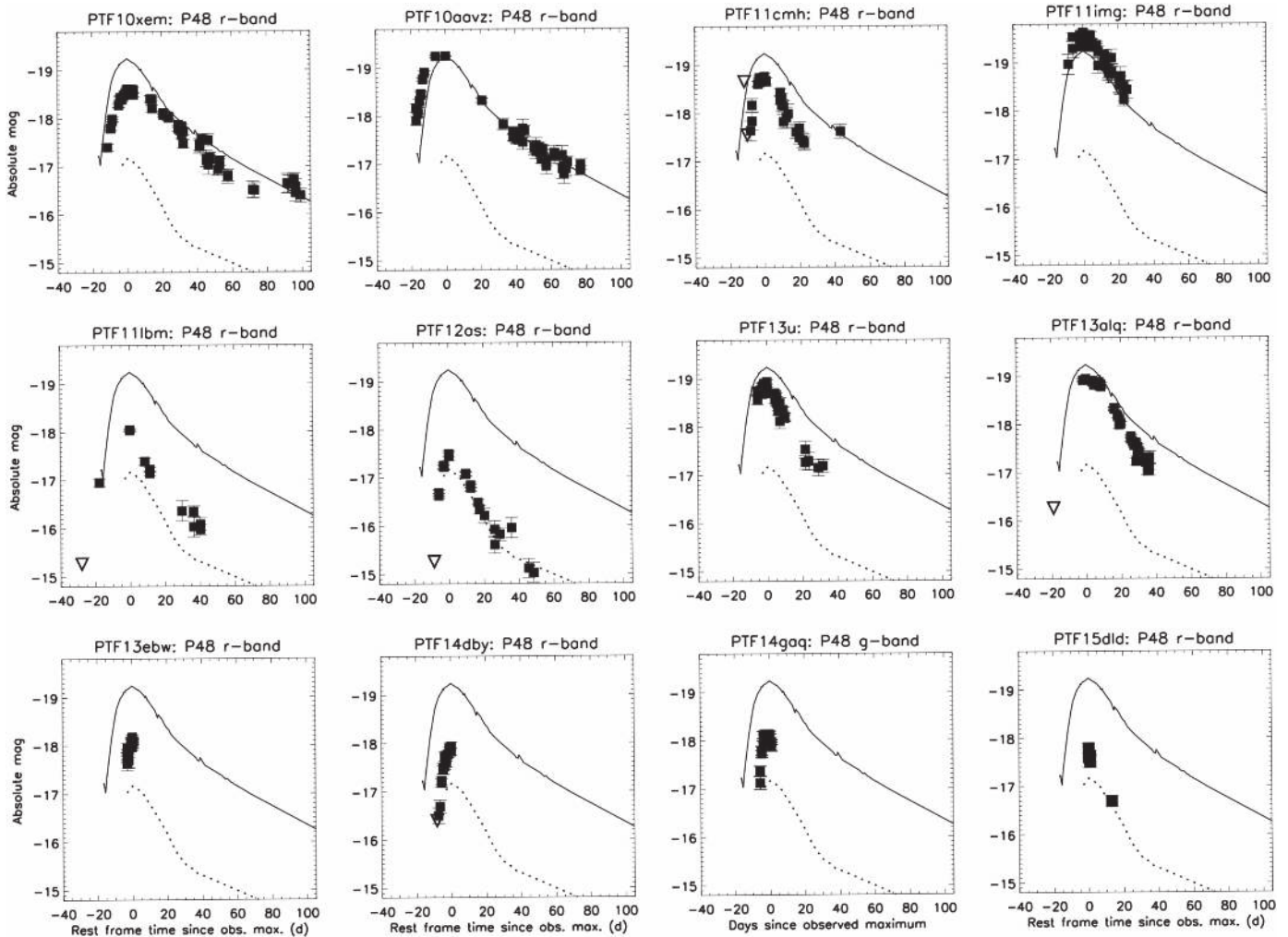
Figure 1. The P48 R - or g -band light curves (corrected for Galactic extinction) of the BL-Ic SNe in our sample. PTF names are reported in the title of each panel. For comparison, we also show the r -band light curve of the GRB-associated BL-Ic SN 1998bw (solid line; Clocchiatti et al. 2011), and of the “ordinary” BL-Ic SN 2002ap (dotted line; Pandey et al. 2003). Epochs on the x -axis are measured since the time of maximum emission as observed by P48 (and corrected for redshift effects). Note that the time of maximum as observed by P48 is different from the SN light curve peak time for cases in which the peak emission was not observed by P48.
