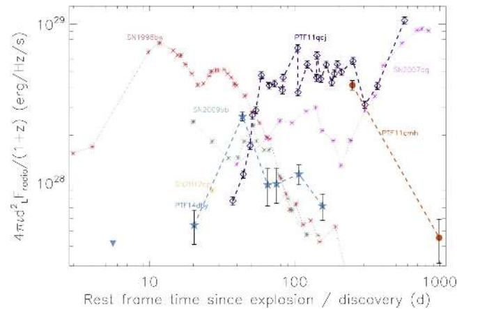
Figure 5. BL-Ic SNe in our sample with radio detections: PTF11cmh (orange dots); PTF11qej (purple diamonds; Corsi et al. 2014); and PTF14dbj (blue stars). We compare these non-relativistic / CSM-interacting SNe with the light curves of the GRB-SN 1998bw (red asterisks; Kulkarni et al. 1998), of the relativistic BL-Ic SN 2009bb (green asterisks; Soderberg et al. 2010), of the CSM-interacting BL-Ic SN 2007bg (magenta asterisks; Salas et al. 2013), and of the relativistic SN 2012ap (yellow asterisk; Chakraborti et al. 2015). As evident from this comparison, the non-relativistic and CSM-interacting BL-Ic peak at later timescales than the relativistic ones.
