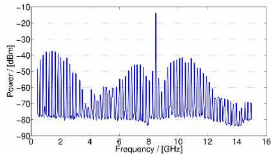
Fig.5. Measured up-converted spectrum at the output of the fiber link. The monocycle is present at baseband and around the local oscillator at f_{LO}=8.5 GHz.
