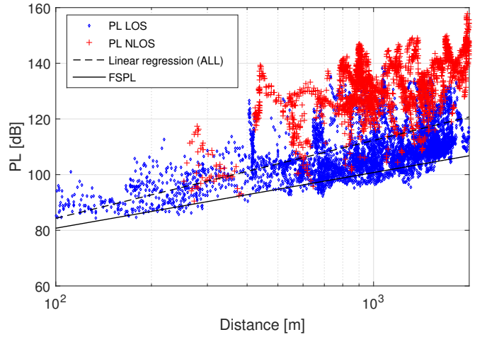
Fig. 7. Path loss and linear regressions considering LOS and NLOS samples, for all Macro Cell transmitters in the hillside mine (2).
