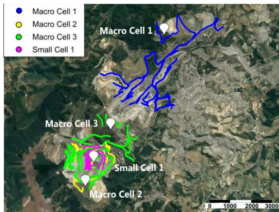
Fig. 1. Measurement routes and transmitter locations at mine 1. The scale is in meters.
