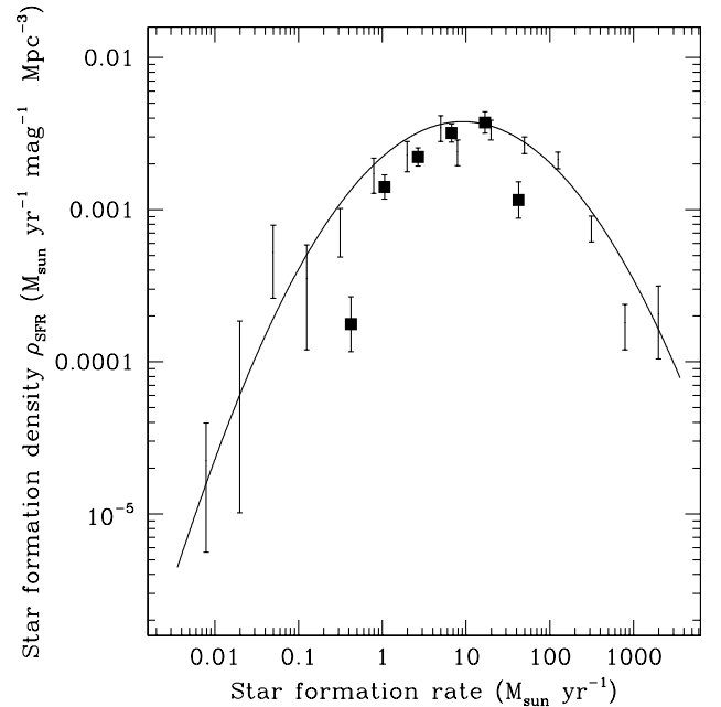
Figure 17. Local star formation density (in M_{\odot} \text{yr}^{-1} \text{mag}^{-1} \text{Mpc}^{-3} ) for galaxies with star formation rates between 0.01 and 1000 M_{\odot} \text{yr}^{-1} . The solid line is derived from the fit to the local RLF for star-forming galaxies (Table 8) after correcting for spectroscopic incompleteness. Error bars from the individual data points used to derive the fit are also shown. Filled squares show the values of local star formation density derived from \text{H}\alpha measurements by Gallego et al. (1995).
