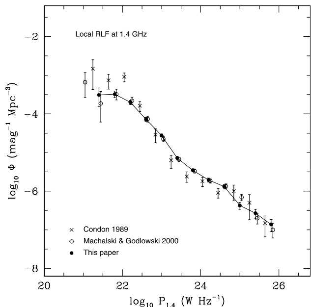
Figure 14. Local RLF derived from the 662 galaxies in Table 1 that are accepted as correct IDs and have radio flux density S_{1.4} \geq 2.8 mJy, optical magnitude 14.0 \leq b_J \leq 19.4 and redshift 0.001 < z < 0.3 . Previous derivations by Condon (1989) and Machalski & Godlowski (2000) are shown for comparison. Between 10^{22} and 10^{24} \text{ W Hz}^{-1} , our values and those of Machalski & Godlowski are sometimes so close that they are indistinguishable in the diagram.
