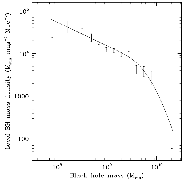
Figure 19. Local mass density (in M_{\odot} \text{ mag}^{-1} \text{ Mpc}^{-3} ) of black holes, derived from the local radio luminosity function for AGN (Tables 7 and 8), together with the mean relation between radio power and black hole mass from Franceschini et al. (1998). As in Fig. 17, error bars are shown for the individual points used to derive the fit in Table 8.
