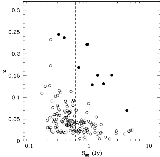
Figure 9. Plot of IRAS 60- \mu\text{m} flux density versus redshift for IRAS -detected 2dFGRS radio sources. ULIRGs with L_{\text{FIR}} > 10^{12} L_{\odot} are shown by filled circles, and other galaxies by open circles. The vertical line at 0.6 Jy corresponds to the flux limit of the PSCz survey (Saunders et al. 2000).
