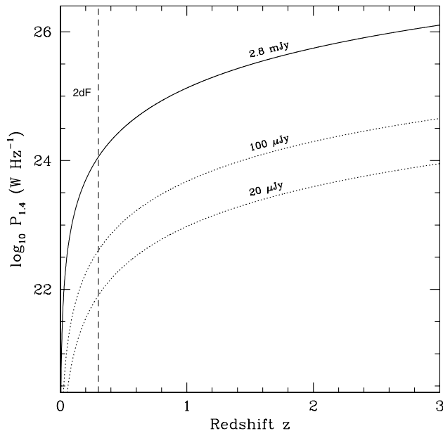
Figure 21. Radio luminosity limits at high redshift for NVSS (2.8-mJy limit) and deeper 1.4GHz surveys (100- and 20- \mu\text{Jy} limits). The vertical line at z = 0.3 marks the effective redshift limit of the 2dFGRS. Note that at z \sim 1 , the deepest surveys so far carried out detect galaxies with radio luminosities above about 10^{23} \text{ W Hz}^{-1} , i.e., in the regime where we expect a mixture of AGN and star-forming galaxies.
