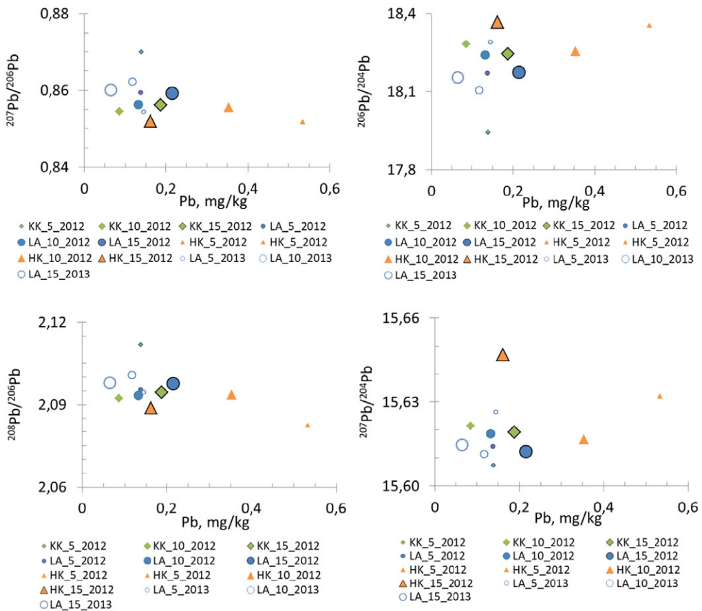
Figure 6 Distribution of Pb isotopic ratio in comparison with lead concentration.
