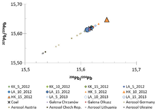
Figure 5 Variation in ^{207}\text{Pb}/^{204}\text{Pb} isotope ratio versus ^{206}\text{Pb}/^{204}\text{Pb} in pine needles (current studies), coal from Katowice, Galena from Olkusz and Chrzanów (De Vleeschouwer et al. 2009) aerosols (after Bollhöfer and Rosman 2001).
