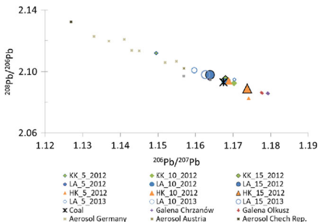
Figure 4 Variation in ^{208}\text{Pb}/^{206}\text{Pb} isotope ratio versus ^{206}\text{Pb}/^{207}\text{Pb} in pine needles (current studies), coal from Katowice, Galena from Olkusz and Chrzanów (De Vleeschouwer et al. 2009), and aerosols (after Bollhöfer and Rosman 2001).
