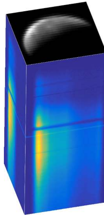
Figure 17. Data cubes from HySICS's in-flight lunar scans provide spectral-radiance as well as spatially integrated irradiance measurements of the Moon (as viewed from the Earth) with improved radiometric accuracy than has as of yet been obtained from Earth-based measurements.
