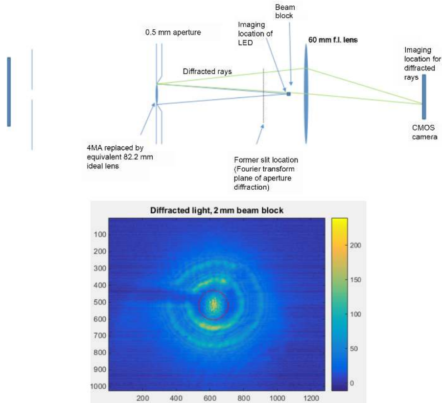
Figure 3. Lab scatter- and diffraction-characterization setup (upper schematic) gives the 2-D pattern shown in the lower image when using a 2 mm beam block behind the 0.5 mm solar-viewing aperture. This beam block occults the un-diffracted and un-scattered light incident on the aperture from a distant, nearly collimated light source (left side of upper schematic). Most light that is diffracted or scattered by the aperture edges passes around the beam block to be reimaged onto the camera, helping to quantify the intensity and spatial pattern of that light. The innermost Airy rings from typical aperture-edge diffraction are visible in the lower image. Since incident sunlight will diffract and scatter similarly, thus spreading some light beyond the edges of the solar-disk image, these effects must be corrected when determining net solar-irradiance values via spatial integrations from HySICS’s cross-slit scans of the solar disk. Lab measurements such as these, combined with diffraction models to account for wavelength sensitivity and extend the spatial extent, help reduce uncertainties for those corrections. (The nearly horizontal radially extending dark region to the left of image center in the lower image is due to the support for the beam block.)
