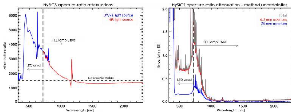
Figure 8. Different illuminations of the optical surfaces by the 0.5 and 20 mm apertures, mainly being affected by a boundary between grating blaze regions, cause the spectrally dependent attenuations that differ from the nominal geometric-ratio value due to the aperture-attenuation method, as shown in the left panel. The blue and the red curves are based on different lab light sources that provide peak power at shorter and longer wavelengths, respectively. The right panel gives the uncertainties in these attenuations. The large peak in uncertainties between the two light sources used is due to low signals from each and could be improved with additional calibration light sources.
