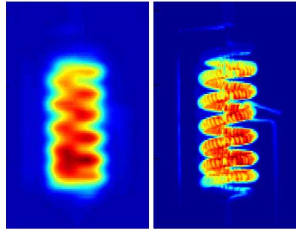
Figure 2. These scans of a lab FEL-lamp filament show the blurring caused by diffraction when using the 0.5 mm aperture (left panel) vs. the 20 mm aperture (right panel). These effects must be accounted for in spatially integrated spectral solar irradiance determinations.
