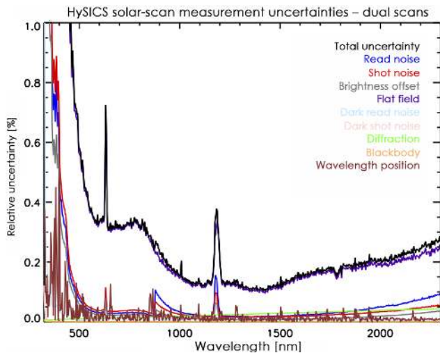
Figure 6. Contributions to net relative uncertainty (black) when observing the Sun during Flight 2 are shown as a function of wavelength. With the exception of the flat-field uncertainties, these plotted uncertainties are the result of two consecutive cross-slit solar scans acquired using specific integration times for the short- and long-wavelength spectral regions to reduce the uncertainties within each. Flat-field uncertainties due to low signal levels dominate across the spectrum but could be reduced with similar multi-image, dual-scan techniques applied to those calibrations.
