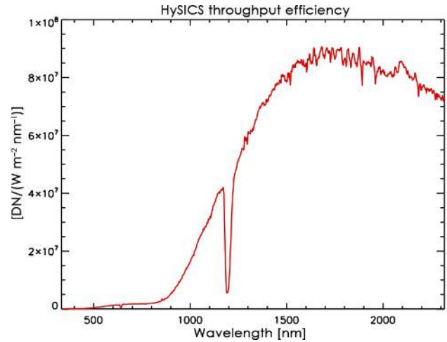
Figure 14. Dividing the HySICS-measured spectral solar irradiance by the modeled SSI in Fig. 13 gives the effective end-to-end sensitivity of the instrument with SI-traceability via correction factor C(\lambda) . This cross calibration can then be applied to Earth ground-scene observations after correcting for the HySICS’s attenuations applied via factor A(\lambda) to provide SI-traceable shortwave-reflected Earth radiances via Eq. (1).
