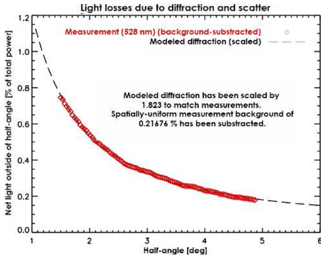
Figure 4. An idealized model estimating the net amount of light falling outside of various angles due to diffraction alone (black dashed curve) is scaled to match lab measurements including both scatter and diffraction (red diamonds) at 528 nm. The measurements match the angular dependence expected from diffraction, indicating that the majority of this measured light loss is mainly due to diffraction rather than scatter, which would have a less-well-modeled relation to angle. Correcting for light losses via this validated diffraction model reduces the uncertainties in solar-radiance measurements, improving the HySICS's determination of spectral solar irradiance.
