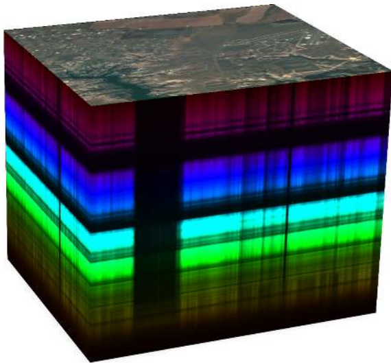
Figure 16. This representation of a three-dimensional data cube is from a ground-scene scan over mixed desert and water to show the generic HySICS data products of spatial/spectral imagery.
