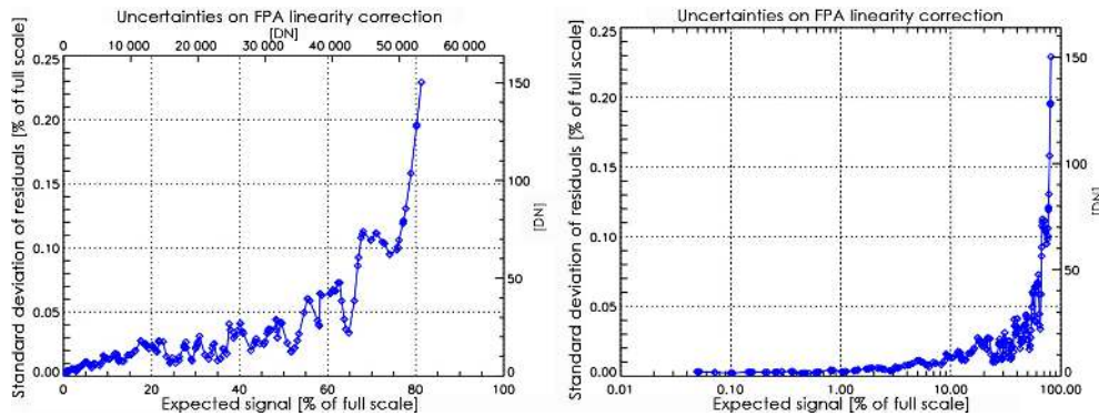
Figure 10. The standard deviations of the residuals from the average of the residuals shown in Fig. 9 indicate the uncertainties in the applied linearity correction as a function of signal level (left panel). The semi-log plot of the same data demonstrates the full > 10^3 measured intensity range (right panel).
