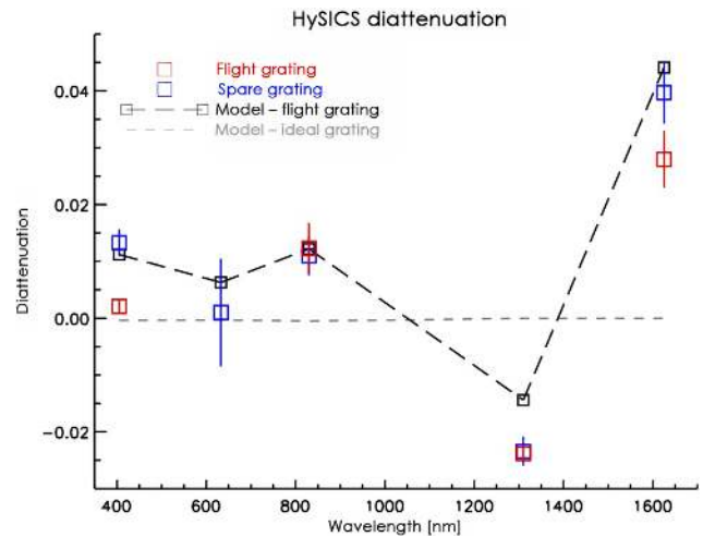
Figure 5. Diattenuation of the HySICS at the integrated-instrument level is limited by high grating-induced polarization, which is as large as 4 % at wavelengths above 1000 nm. A Zemax model based on the flight-grating measurements (black, long dashes) shows the lower instrument diattenuations expected using a less-polarization-sensitive grating (gray, short dashes).
