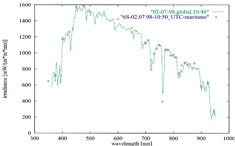
Fig. 9: Comparison of computed (◇) and measured irradiance (solid line -) at 10:48 GMT with optical thickness \tau=0.34
