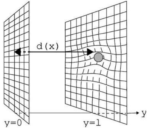
FIG. 1. Radion as a distance between two branes.
