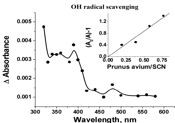
Figure 3. Difference in absorption spectrum of the transient obtained on pulse radiolysis of N 2 O saturated aqueous solutions containing 100µg/ml of PAE (methanolic extract of Prunus avium fruits) at pH 7. Inset shows linear plot for competition kinetics between SCN 2- and PAE towards hydroxyl radicals. Lines show fitting according to equation 3.
