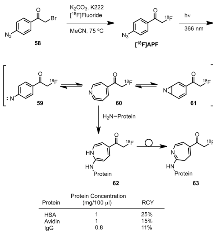
Scheme 28. Photochemical Reactions with Fluorine-18
