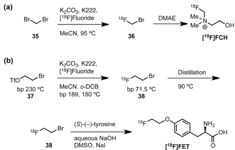
Scheme 22. Radiosynthesis of (a) [^{18}\text{F}]\text{FCH} and (b) [^{18}\text{F}]\text{FET}
