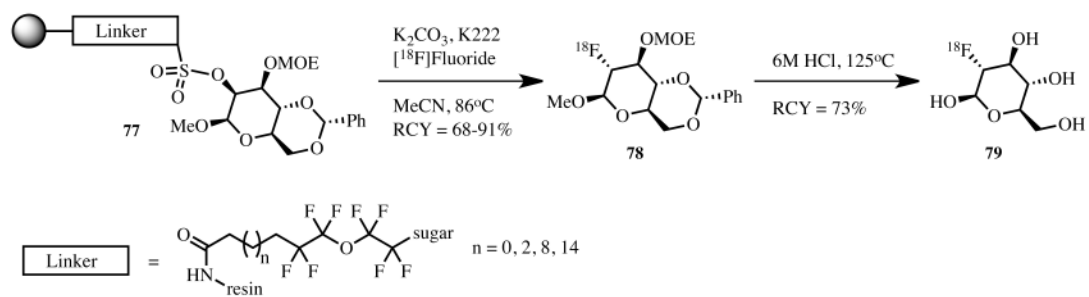
Scheme 34. Solid-phase Synthesis of [ ^{18}\text{F} ]FDG
