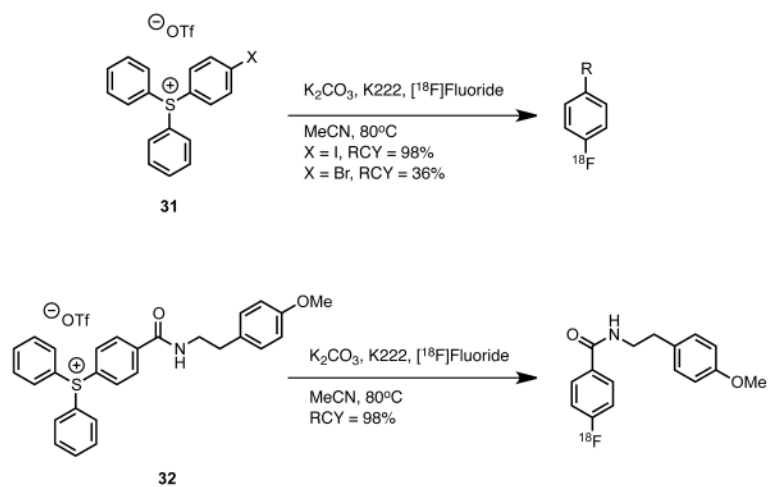
Scheme 19. [ ^{18}\text{F} ]Fluoroarenes from triarylsulfonium salts.
